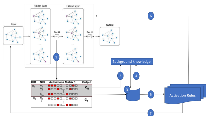
Fig. 2. INSIDE-GNN Process: Sequential Discovery and Integration of Activation Rules for Enhanced Model Insight
