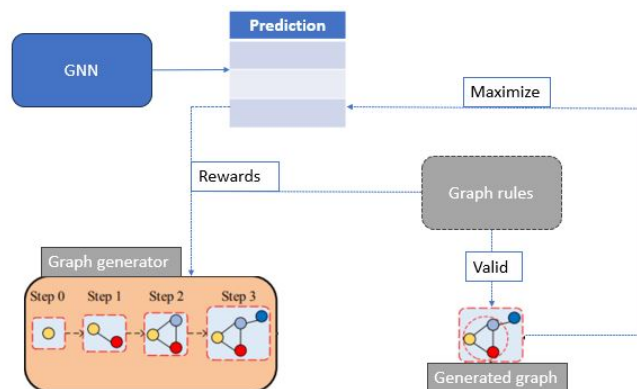
Fig. 3. The architecture of GraphLIME
