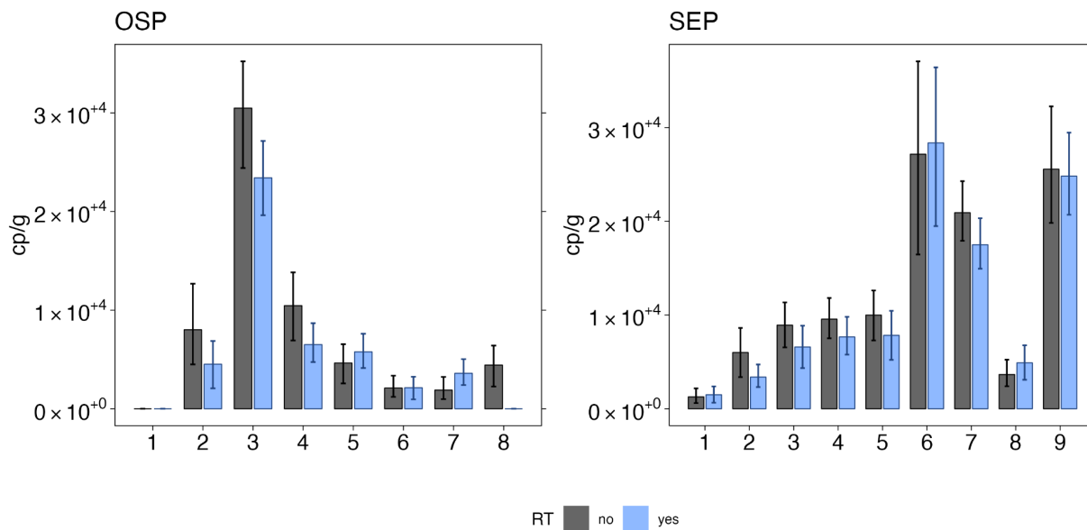
414 415 Fig 3. Comparison of HIV nucleic acid quantification with and without RT. Concentrations 416 of HIV nucleic acids in wastewater solids from OSP and SEP are expressed in terms of copies 417 of the target per gram dry weight of solids found in wastewater for quantification with the use of 418 RT (blue) and without (black). Errors on each bar represent standard deviations (68% 419 confidence intervals) from the droplet digital RT-PCR measurement and include Poisson error 420 as well as variation among replicate wells. 421
