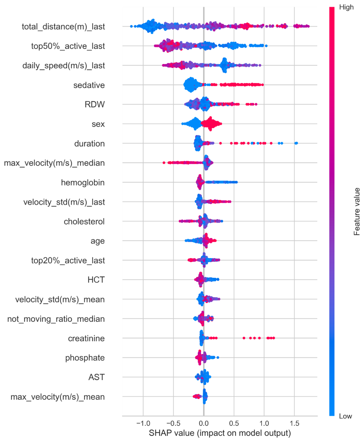
Fig. 4. Visualizing feature importance for the combined clinical + RTLS model using SHAP values.
