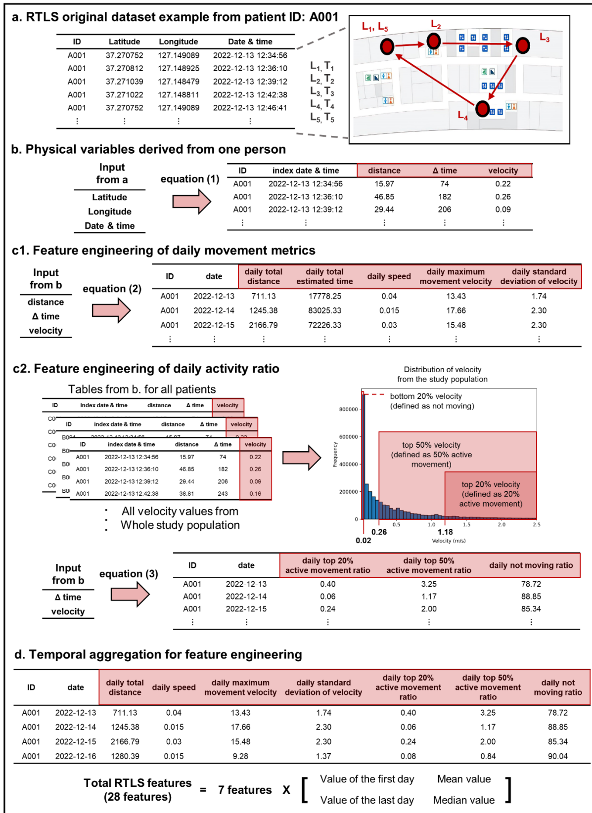
Fig. 6. Overall flow of RTLS feature engineering.
