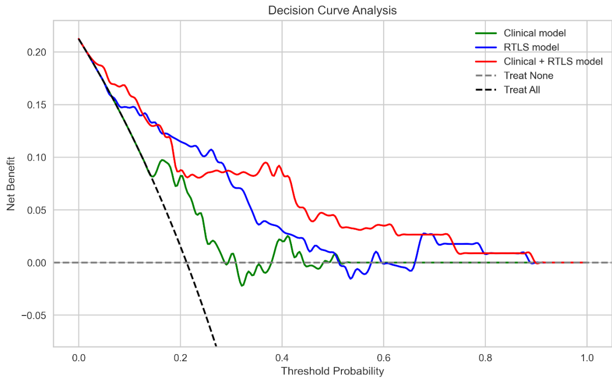
Fig. 5. DCA of each model performance.
