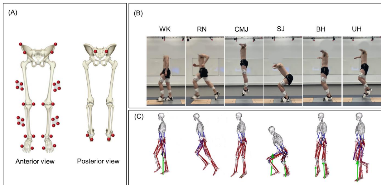
Fig. 1. Marker set for motion capture data and Musculoskeletal models. Twenty-two individual markers and four cluster markers were placed on the bone anatomical landmarks of the lower body (A). Six different exercises; walking, running, countermovement jump, squat jump, unilateral hopping, and bilateral hopping, were performed by each participant (B). Scaled Musculoskeletal models were developed in OpenSim representing each performed exercise (C).
