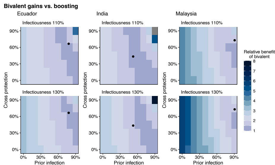
Figure 4: Comparison of bivalent vs. monovalent boosters in the HIM. Relative benefit of the bivalent booster is calculated with Equation 1, matching the HSM. Grey values represent high-immunity areas where zero deaths were averted by a monovalent booster and thus Equation 1 cannot be calculated. Prior immunity represents the percentage of the population that has been previously infected. Cross protection represents the overlap between the population's immune history and the currently circulating variant. Country-specific immunity levels are included (black dots).
