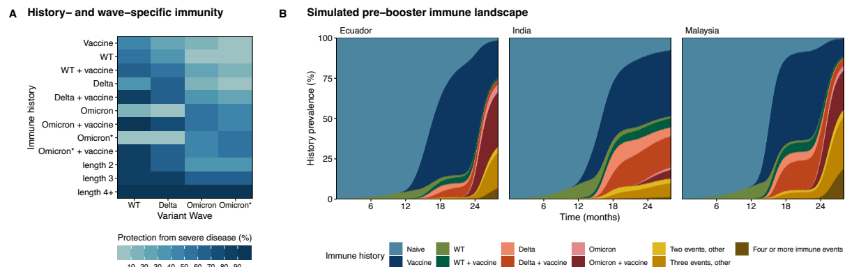
Figure 1: Landscapes of immunity from the history-specific model (HSM). (A) Level of protection from severe disease by immune history and variant wave, estimated using neutralizing antibody titers in human sera [19, 20]. Lengths 2, 3, and 4+ represent permutations of immune history that were not explicitly tracked (e.g. 'WT + Delta + Omicron'). (B) Average immune history trajectories of 500 runs informed by historical incidence data from Ecuador, India, and Malaysia shown in Figure S1 [21]. Simulations of the prevalence of histories are shown until day 839, one day before booster vaccinations are implemented at 28 months. The infections over time for each country are shown in Figure S2. General simulation parameters are shown in Table S3, with country-specific population structure in Table S4, contact rates by country and SES in Table S5, wave- and country-specific stringency in Table S1, and vaccination parameters by country and SES in Table S2. The HSM compartmental diagram is shown in Figure S5.
