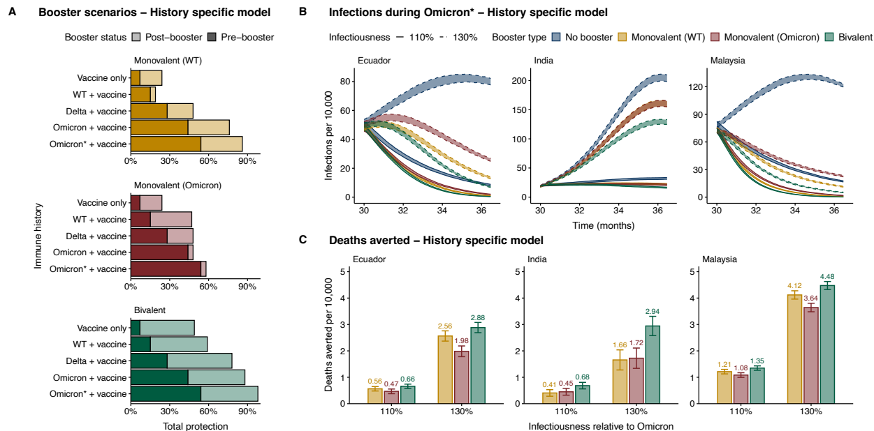
Figure 2: HSM booster parameters and projections during the Omicron* period. (A) Booster protection against severe disease during the Omicron* wave, by immune history, under a bivalent, WT monovalent, or hypothetical Omicron monovalent formulation. (B) Infection trends under three boosters or a no-boosting scenario based on the characteristics of Ecuador, India, and Malaysia. We simulated two scenarios of infectiousness where Omicron* is 10% or 30% more infectious than Omicron. 95% confidence intervals from the t-distribution are shown (ribbons). (C) Deaths averted by boosting since the start of Omicron* (30 months) through the end of simulations, under each booster. 95% confidence intervals from the t-distribution are shown with whiskers. Boosting parameters, which are assumed to be 10 weeks faster than for primary series vaccination, are shown in Table S8.
