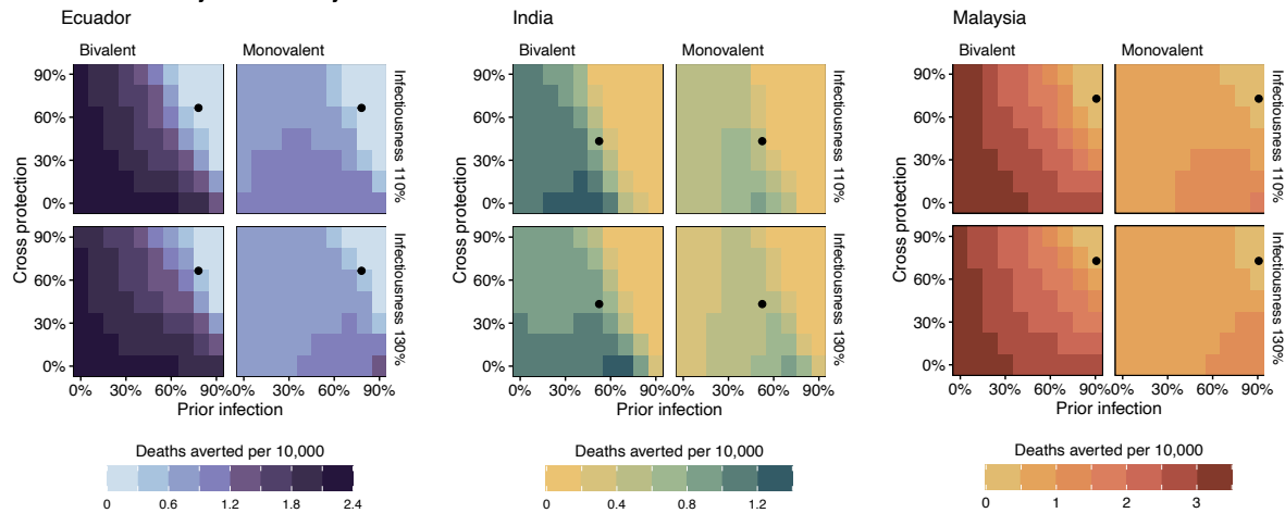
Figure 3: HIM projections. (A) Infections per 10,000 during the Omicron* period, where Omicron* is considered to be 10% or 30% more infectious than Omicron. (B) Deaths averted per 10,000 under a bivalent or monovalent booster, compared to a ‘no boosting’ scenario. Prior immunity represents the percentage of the population that has been previously infected. Cross protection represents the overlap between the population’s immune history and the currently circulating variant. Country-specific immunity levels are included (black dots). The HIM model structure is shown in Figure S5. General parameters are shown in Table S3, stringency in Table S1, initial conditions in Table S10, cross-protection in Table S9, and boosting parameters in Table S8.
