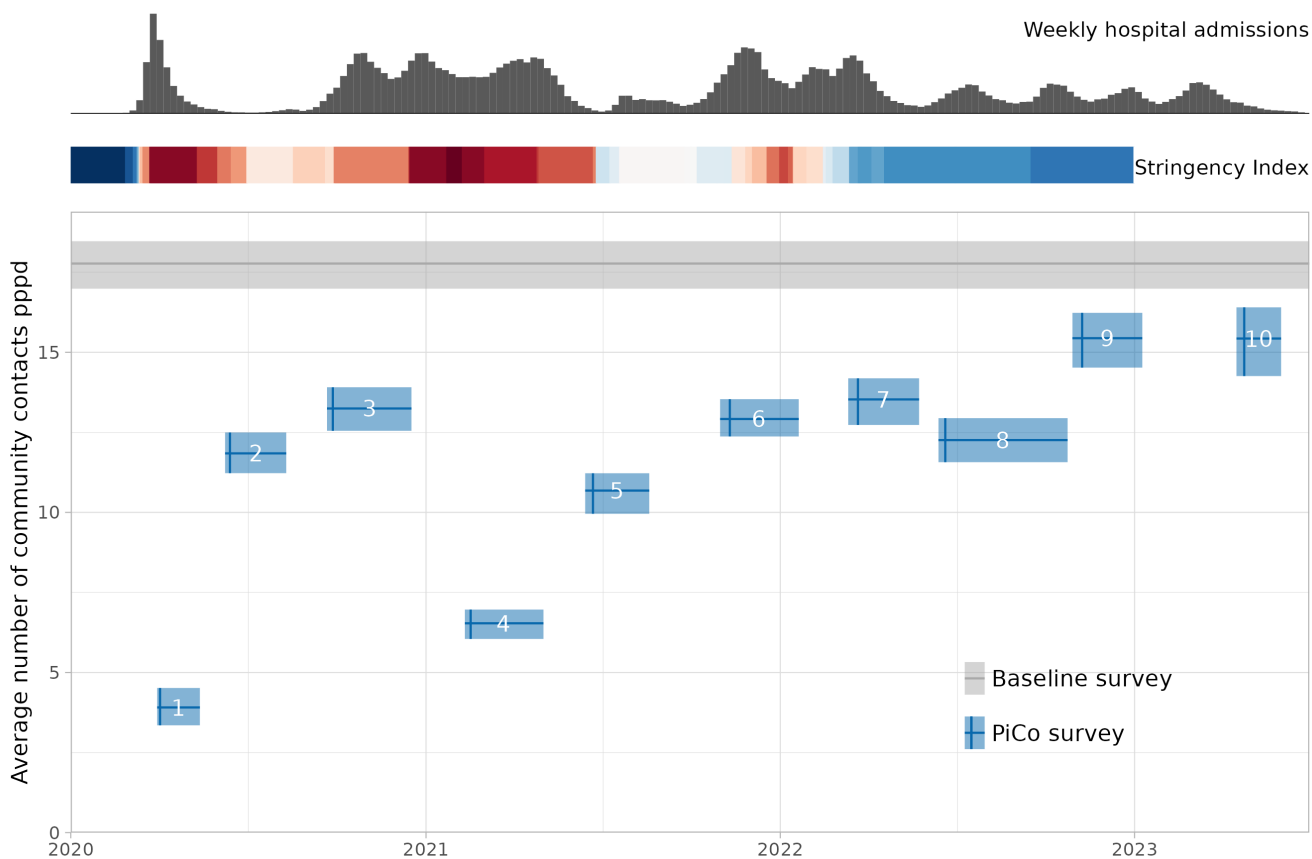
Figure 2: Weighted average number of community contacts per person per day (pppd) in the general population, for the baseline and PiCo survey. Shown is the weighted average number of contacts (horizontal line) and 95% bias-corrected bootstrap interval (shaded area). PiCo rounds are shown from the start to end date, with the median survey date (vertical line) with the survey round number in white. As a timeline reference the weekly number of hospital admissions [38] and the Oxford Stringency Index [39] are depicted on top. The stringency index is color coded from blue (low) to red (high).
