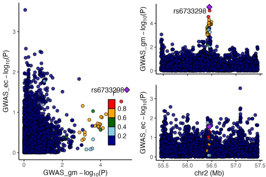
Figure 2. Colocalisation results for lead SNP (rs6733298) associated with the G. unclassified, F. Erysipelotrichaceae P/A microbial trait with endometrioid cancer.
