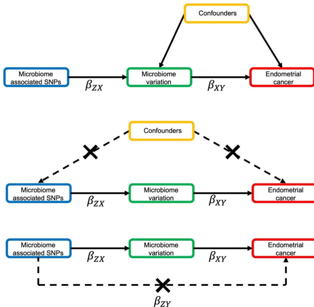
Figure 3. MR framework applied to assess the causal effect of the gut microbiome on endometrial cancer risk
