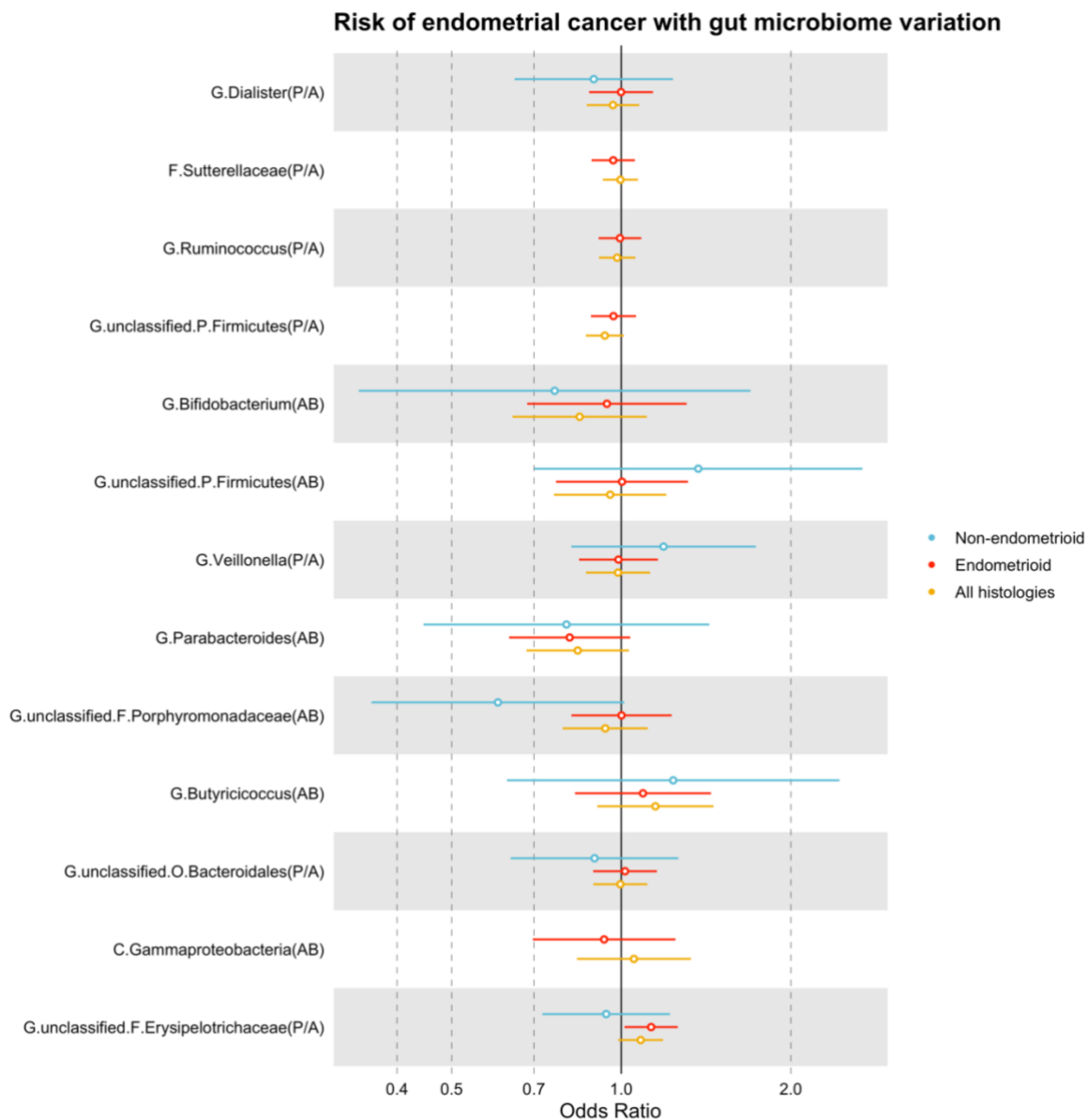
Figure 1. MR estimates of the effect of each microbial trait on endometrial cancer and subtypes.
