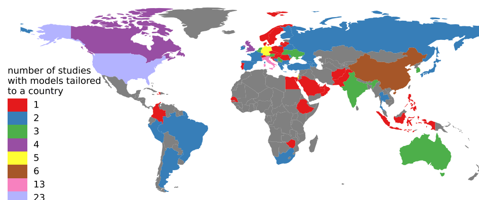
Figure 2: Number of studies that contain a model for a specific country. Some studies include models tailored to several countries, while others are more abstract and not tailored to a specific country. Census data and age-stratified contact matrices are two examples of frequently used country-specific data.
