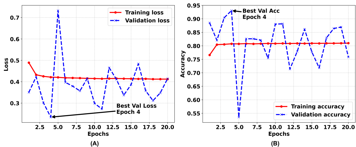
Figure 13. Loss and accuracy of the proposed ANN model with respect to epochs. (A) Visualization of training and validation loss per epoch. (B) Visualization of training and validation accuracy per epoch. The observed changes in the training and validation phases are shown in this section.
