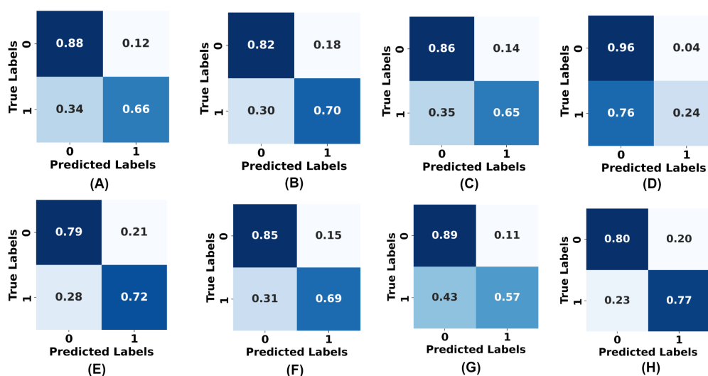
Figure 15. Confusion matrix for all the applied models. (A) Confusion matrix of the Adaptive Boosting model. (B) Confusion matrix of the Random Forest model. (C) Confusion matrix of the Random Under-Sampling model. (D) Confusion matrix of the Decision Tree model. (E) Confusion matrix of the Gaussian Naive Bayes model. (F) Confusion matrix of the Multilayer Perceptron model. (G) Confusion matrix of the Convolutional Neural Network model. (H) Confusion matrix of the proposed Artificial Neural Network model. The representation of correct and incorrect prediction rates for both prediction classes.
