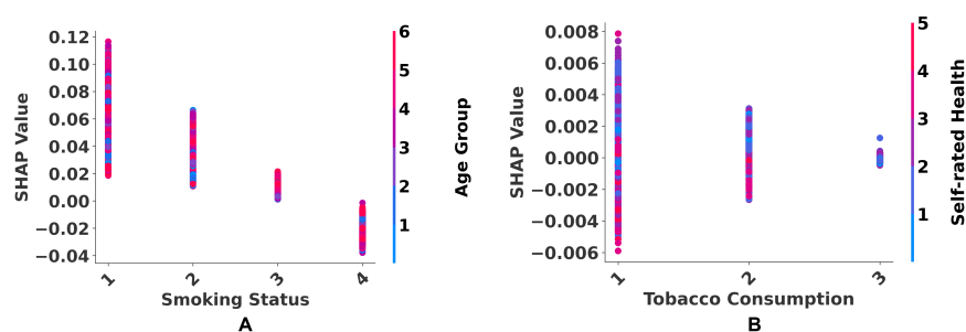
Figure 11. A dependence graphic to represent the predictive effect of each category in personal health habits features with interaction effects. SHapley Additive exPlanations (SHAP) values were employed to represent the effect of each category on personal health habits features in terms of identifying myocardial infarction (MI) probability including the interaction effects with other features. The x-axis represents the different categories inside a specific feature from personal health habits. Besides, the y-axis represents SHAP values for an input category inside that specific feature. The color bar represents different input categories from another feature that interacts with that specific feature.
