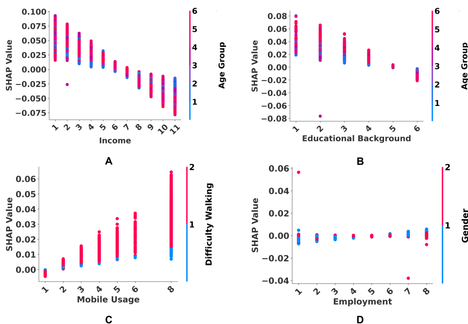
Figure 8. A dependence graphic to represent the predictive effect of each category in economic and social status features with interaction effects. SHapley Additive exPlanations (SHAP) values were employed to represent the effect of each category in economic and social status in terms of identifying myocardial infarction (MI) probability including the interaction effects with other features. The x-axis represents the different categories inside a specific feature from economic and social status. Besides, the y-axis represents SHAP values for an input category inside that specific feature. The color bar represents different input categories from another feature that interacts with that specific feature.
