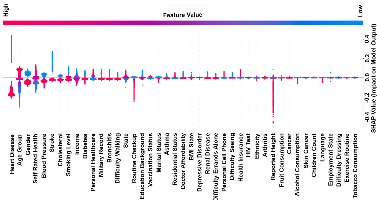
Figure 5. A summary graphic that employs SHapley Additive exPlanations (SHAP) values to combine feature importance and feature effects of the selected features from the preprocessed dataset. The graphic is positioned in a rotated manner. Each point on the x-axis indicates a Shapley value for a particular feature. When it comes to Shapley values, higher values indicate the most significant features and lower values denote fewer significant features. The features are listed in descending order of importance on the y-axis. The color of the dots corresponds to the respective feature categories from the dataset, which range from low to high. Each feature category represents a specific group of individuals.
