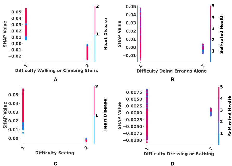
Figure 7. A dependence graphic to represent the predictive effect of each category in impairment status features with interaction effects. SHapley Additive exPlanations (SHAP) values were employed to represent the effect of each category in impairment status in terms of identifying myocardial infarction (MI) probability including the interaction effects with other features. The x-axis represents the different categories inside a specific feature from impairment status. Besides, the y-axis represents SHAP values for an input category inside that specific feature. The color bar represents different input categories from another feature that interacts with that specific feature.
