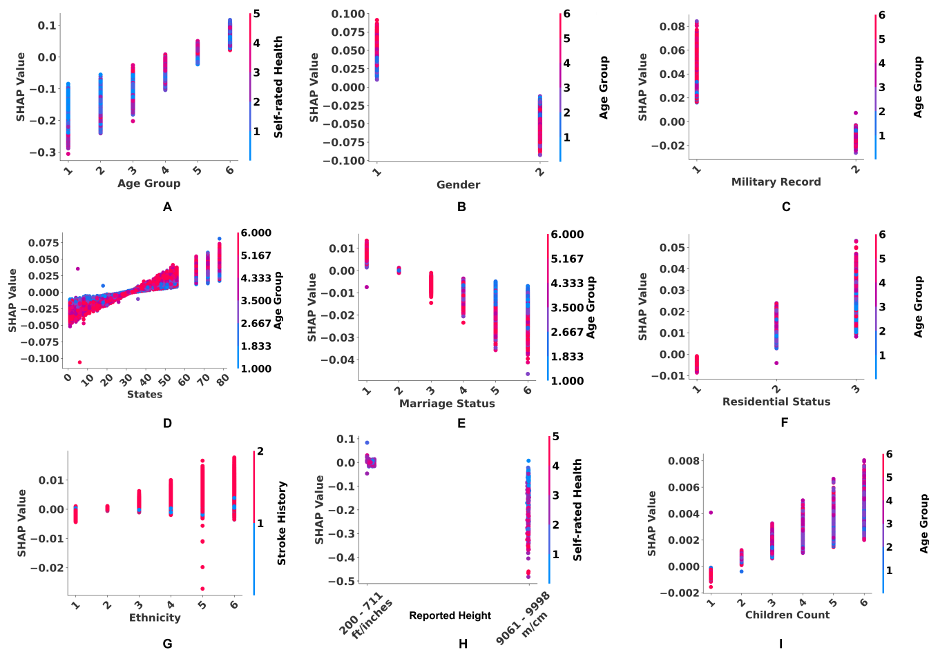
Figure 10. A dependence graphic to represent the predictive effect of each category in socio-demographic features with interaction effects. SHapley Additive exPlanations (SHAP) values were employed to represent the effect of each category in socio-demographic features in terms of identifying myocardial infarction (MI) probability including the interaction effects with other features. The x-axis represents the different categories inside a specific feature from socio-demographics. Besides, the y-axis represents SHAP values for an input category inside that specific feature. The color bar represents different input categories from another feature that interacts with that specific feature.
