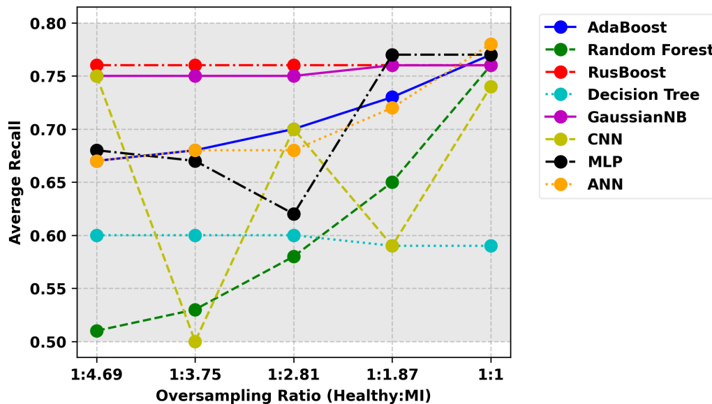
Figure 12. Average recall for all the applied models across each oversampled trainset using Minority-weighted Sampling. Minority class (MI cases) in the train data were oversampled at different ratios using Minority-weighted Sampling and multiple approaches were employed to measure the optimal model for achieving the best outcomes across the given distributions.
