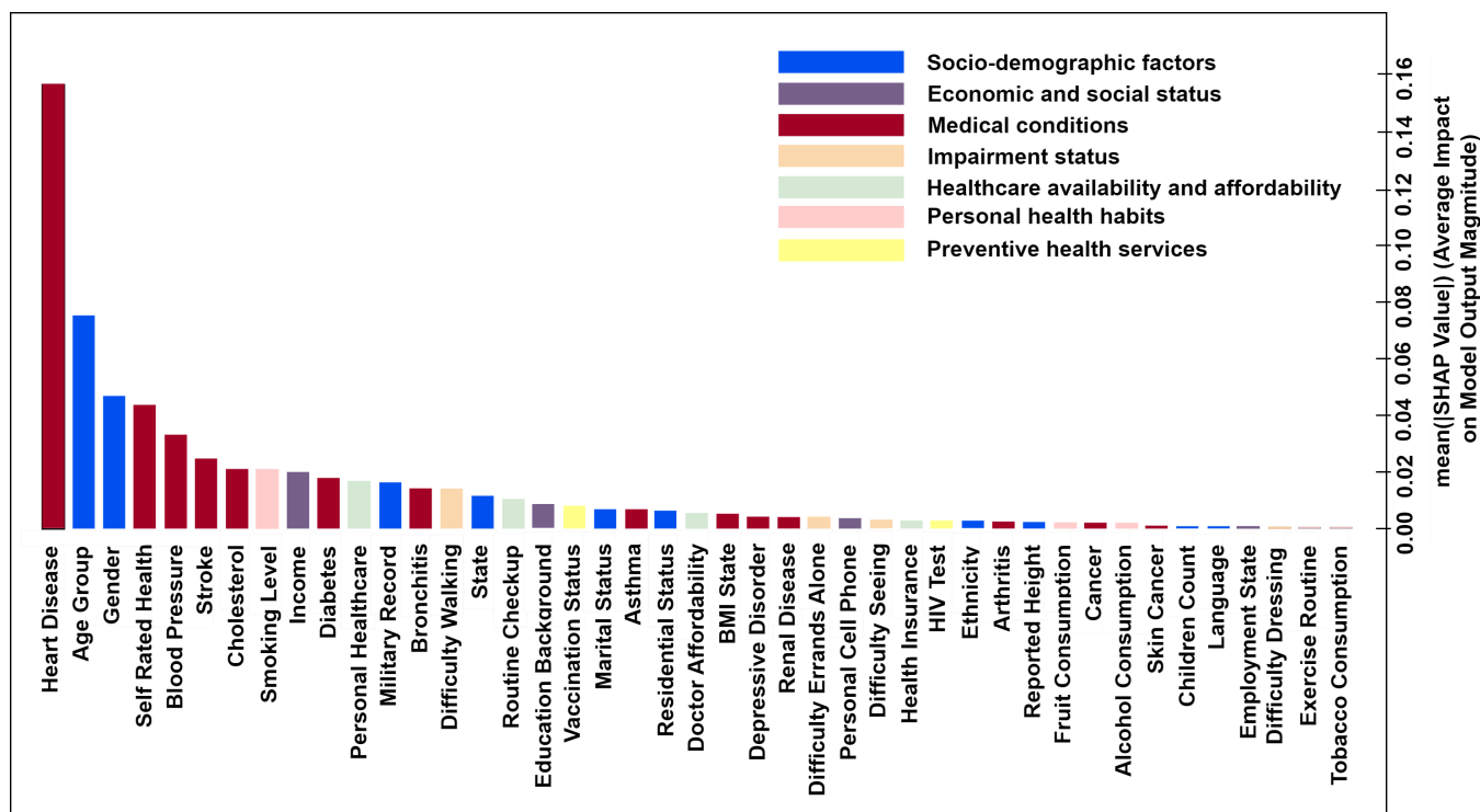
Figure 4. Feature importance employing SHapley Additive exPlanations (SHAP) values using the proposed Artificial Neural Networks (ANN) model. The significance of each feature from specified input domains toward prediction was shown in this section. Each color shade represents an input domain. The features are listed in descending order of importance.
