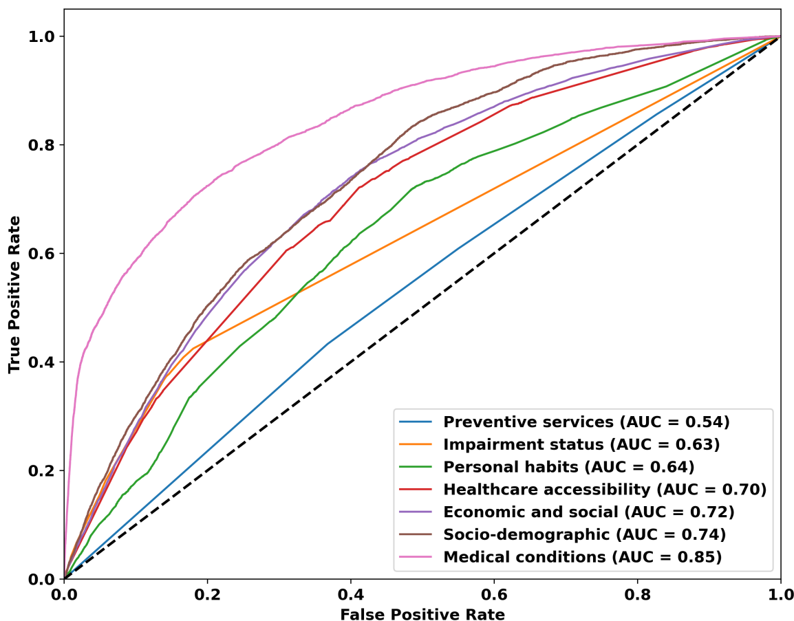
Figure 3. Area Under the Receiver Operating Characteristic (ROC) curve for the selected features from specific input domains using the proposed Artificial Neural Networks (ANN) model. AUC curves for each input domain are implemented in this section to demonstrate the true positive and false positive rates.
