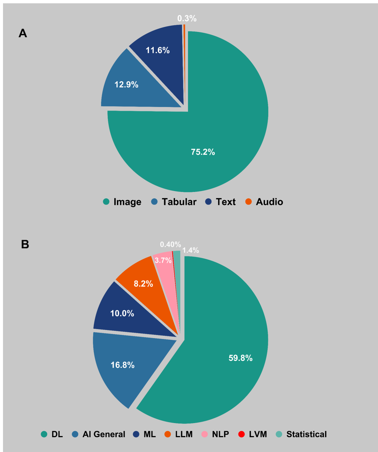
Figure 4: A) Distribution of data types utilized in the mature articles in the year 2023. B) Distribution of model types utilized in the mature articles in the year 2023, where DL = Deep Learning, ML = Machine Learning, LLM = Large Language Models, NLP = Natural Language Processing, LVM = Large Vision Models.
