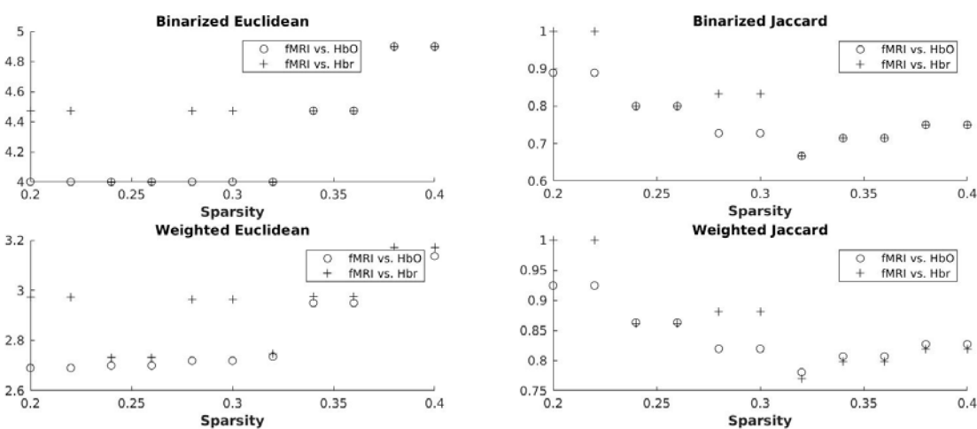
Figure 2. Similarity of RSFC maps between fNIRS and fMRI with sparsity, measured by Euclidean distance on binarized maps (upper left), Euclidean distance on weighted maps (lower left), Jaccard distance on binarized maps (upper right), and Jaccard distance on weighted maps (lower right).
