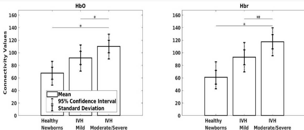
Figure 4. Very preterm born neonates scanned at term-equivalent age showed increased HbO (left) and Hbr (right) connectivity values relative to healthy newborns and neonates with mild IVH. ** p < 0.01 , * p < 0.05 .
