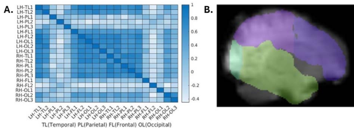
Figure 1. A. Connectivity matrix for the signals extracted from the fNIRS channels in the left (LH) and right (RH) hemispheres from the temporal, parietal, frontal and occipital lobes. B. Lobe-based analysis of the fMRI data. A hemisphere is sectioned into temporal, parietal, frontal and occipital lobes.
