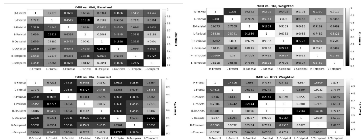
Figure 3. Lobe-wise similarity maps at sparsity of 32%. Higher values reflect greater similarity between the two modalities. Average values among channels are 0.5390 (upper left), 0.5260 (lower left), 0.7031 (upper right) and 0.6761 (lower right).
