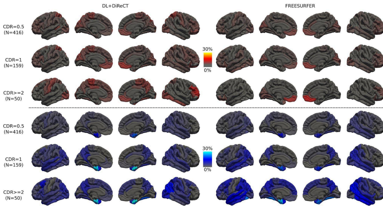
Figure 2: Percentage of CTh anomalies detected by ScanOMetrics in patients with AD, stratified by cognitive impairment levels at scan time (CDR=0.5: rows 1 and 4, CDR=1: rows 2 and 5, and CDR \geq 2: rows 3 and 6). The upper half depicts CTh increase, while the lower half shows progression of CTh reduction. Mind that the color scales are different from the ones used in Figure 1.
