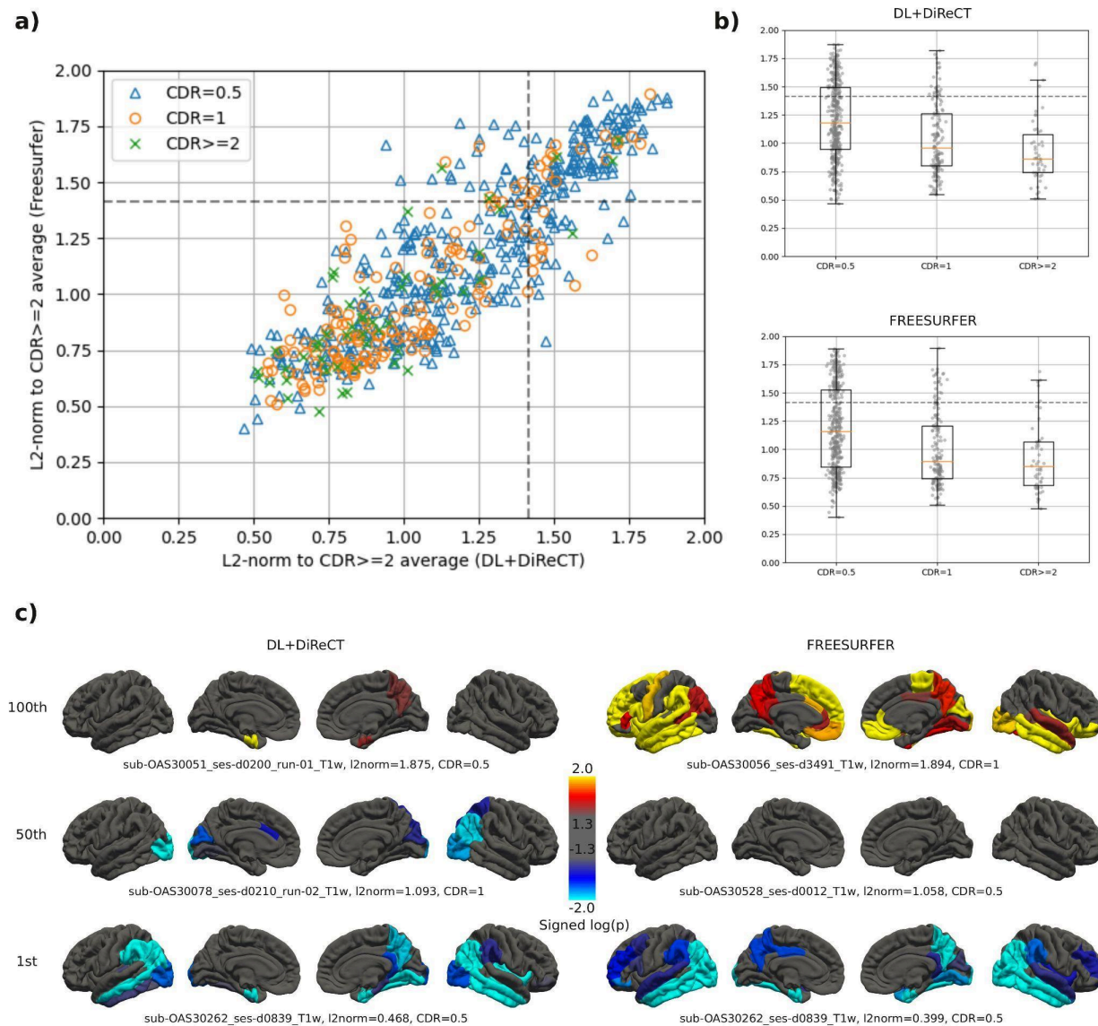
Figure 3: Normalized L2-distances between individual significance maps and a template (i.e. the average map of all scans with CDR \geq 2). Significance maps are log 10 (p) maps with negative sign for CTh reduction and positive sign for CTh increase. Normalized L2-distances range from 0 for identical maps to 2 for antisymmetric maps, with \sqrt{2} indicating orthogonal maps (marked by dotted lines in panels a and b). a) Correlation between DL+DiReCT and FreeSurfer, individual CDR scores are symbol/color coded. b) Grouping by CDR separately for both software tools. c) Significance maps in individual scans, selected according to their L2-distance. Scans on the 1st row are the 100th percentiles in the distributions (i.e. highest distance to the reference), while the lowest row are the most similar to the group average. In the lowest row the same scan was selected for both DL+DiReCT and FreeSurfer, and corresponds to the data point closest to the origin in panel a).
