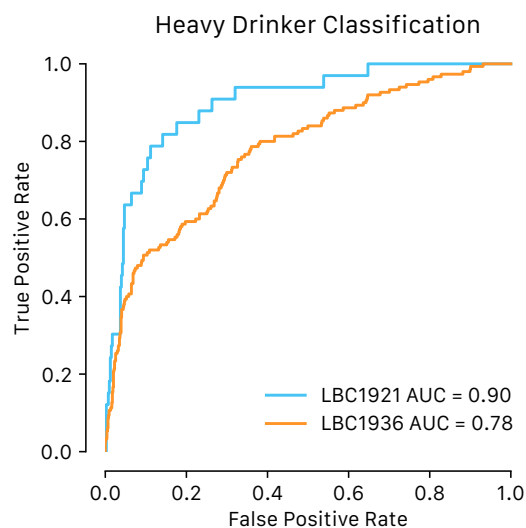
Figure 2. AUC analysis of alcohol consumption prediction in the Lothian Birth Cohorts of 1921 and 1936. Shown are area under the receiver operating characteristic curves for classifying dichotomized alcohol consumption (heavy drinkers - >14 units per week for females or >21 units per week for males - versus non- or light-moderate drinkers).
