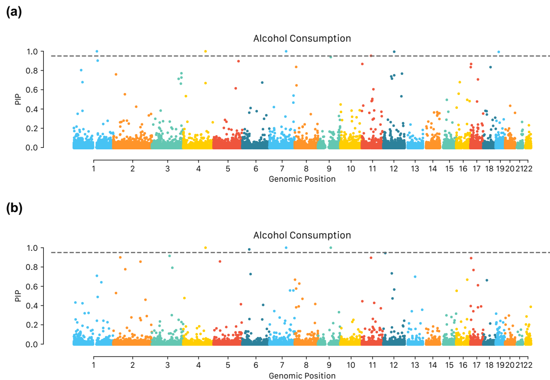
Figure 3. EWAS of alcohol consumption Manhattan plot. Model using 1) usual drinkers and 2) full cohort. Threshold line set at posterior inclusion probability (PIP) = 0.95.
