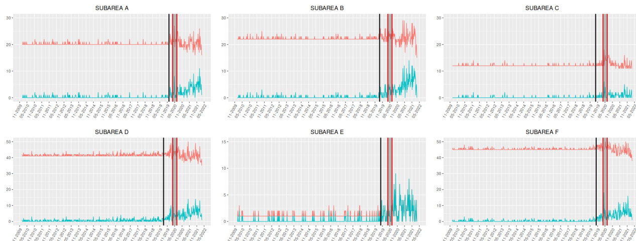
Figure 5: Evolution of the weekly number of GBV diagnoses in each subarea of the Àmbit Metropolità Nord (Catalonia, Spain) (in green) and a reconstruction of the most likely process according to Eq. (2) (in red) for scenario 2. The solid black vertical line indicates the moment when training starts to impact the underreporting process, while the area between the red vertical lines represents the confinement period.
