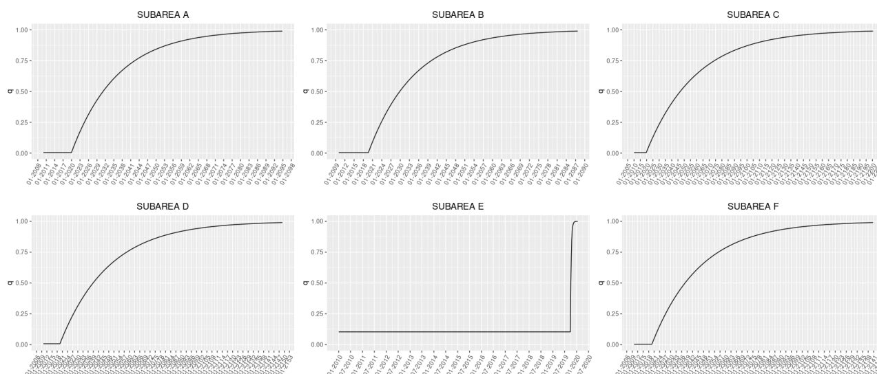
Figure 9: Evolution of \hat{q}_t in each subarea according to scenario 3.
