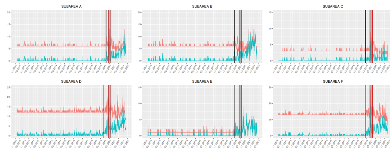
Figure 2: Evolution of the weekly number of GBV diagnoses in each subarea of the Àmbit Metropolità Nord (Catalonia, Spain) (in green) and a reconstruction of the most likely process according to Eq. (2) (in red) for scenario 1. The solid black vertical line indicates the moment when training starts to impact the underreporting process, while the area between the red vertical lines represents the confinement period.
