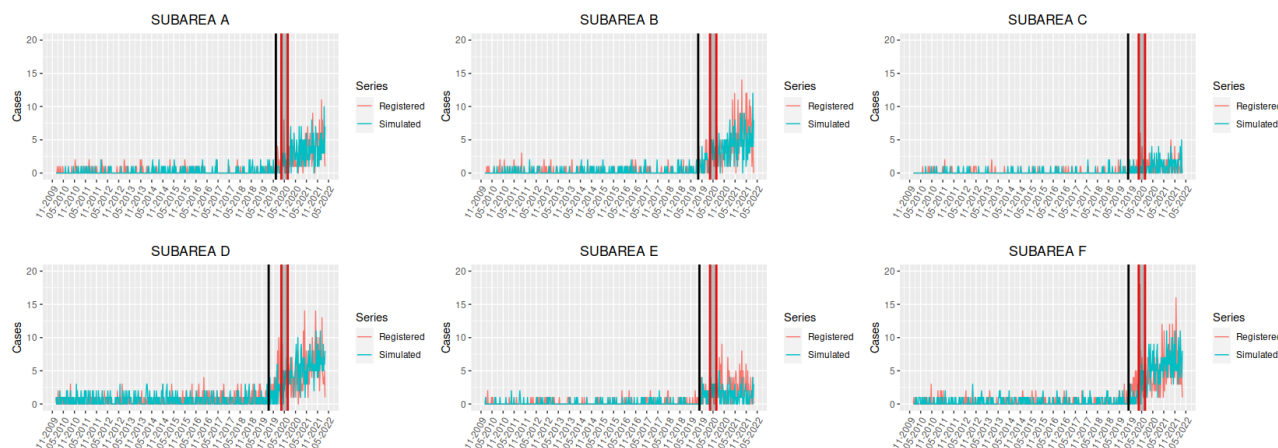
Figure 1: Evolution of the weekly number of GBV diagnoses in each subarea of the Àmbit Metropolità Nord (Catalonia, Spain) (in red) and estimated observed process according to the theoretical model (in green) for scenario 1. The solid black vertical line indicates the moment when training starts to impact the underreporting process, while the area between the red vertical lines represents the confinement period.
