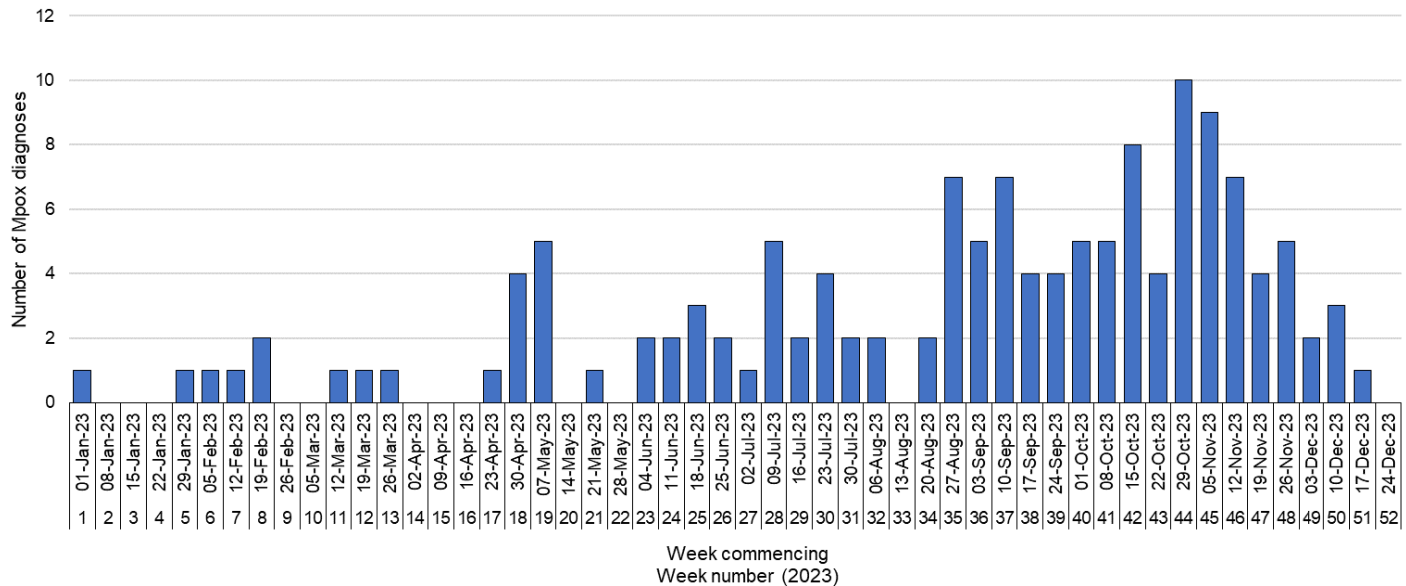
Figure 1. Confirmed and highly probable mpox cases by week of specimen date in England, 01 January to 31 December 2023
