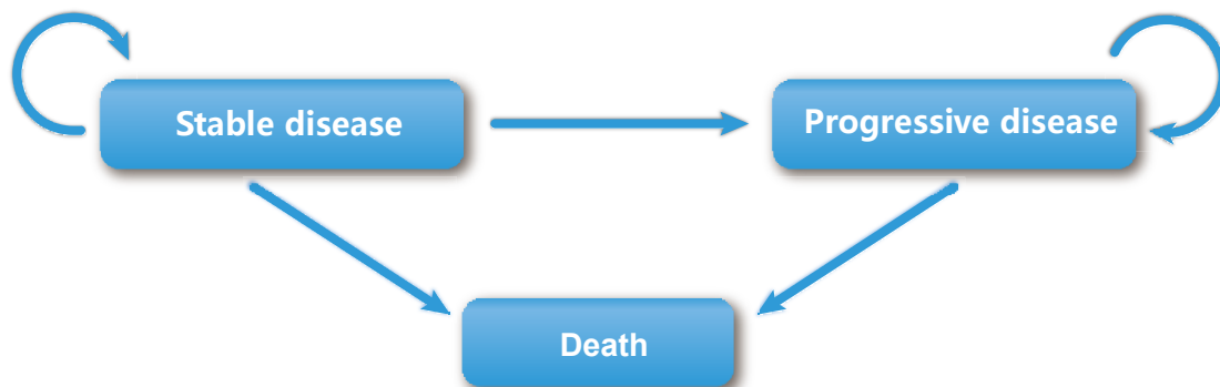
122 Figure 1. Markov state transition model.
