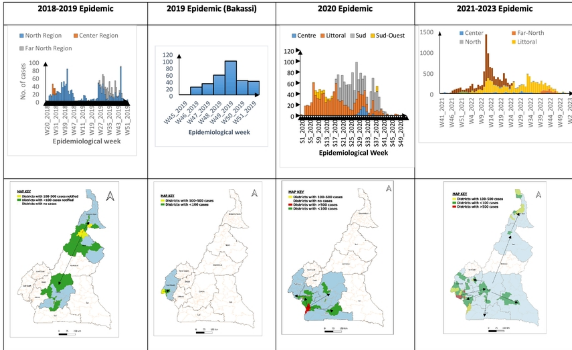
Figure 1: Epidemic curves and geographical distribution of cases by health district of cholera cases during each epidemic from 2018-2023. The maps in the second row indicate the districts affected during the corresponding epidemics indicated in the epidemic curves in the row above. The arrows in the maps indicate the evolution of the spread of cases by region /districts affected. This information was generated from the dates of onset of cases notified in the cholera database.
