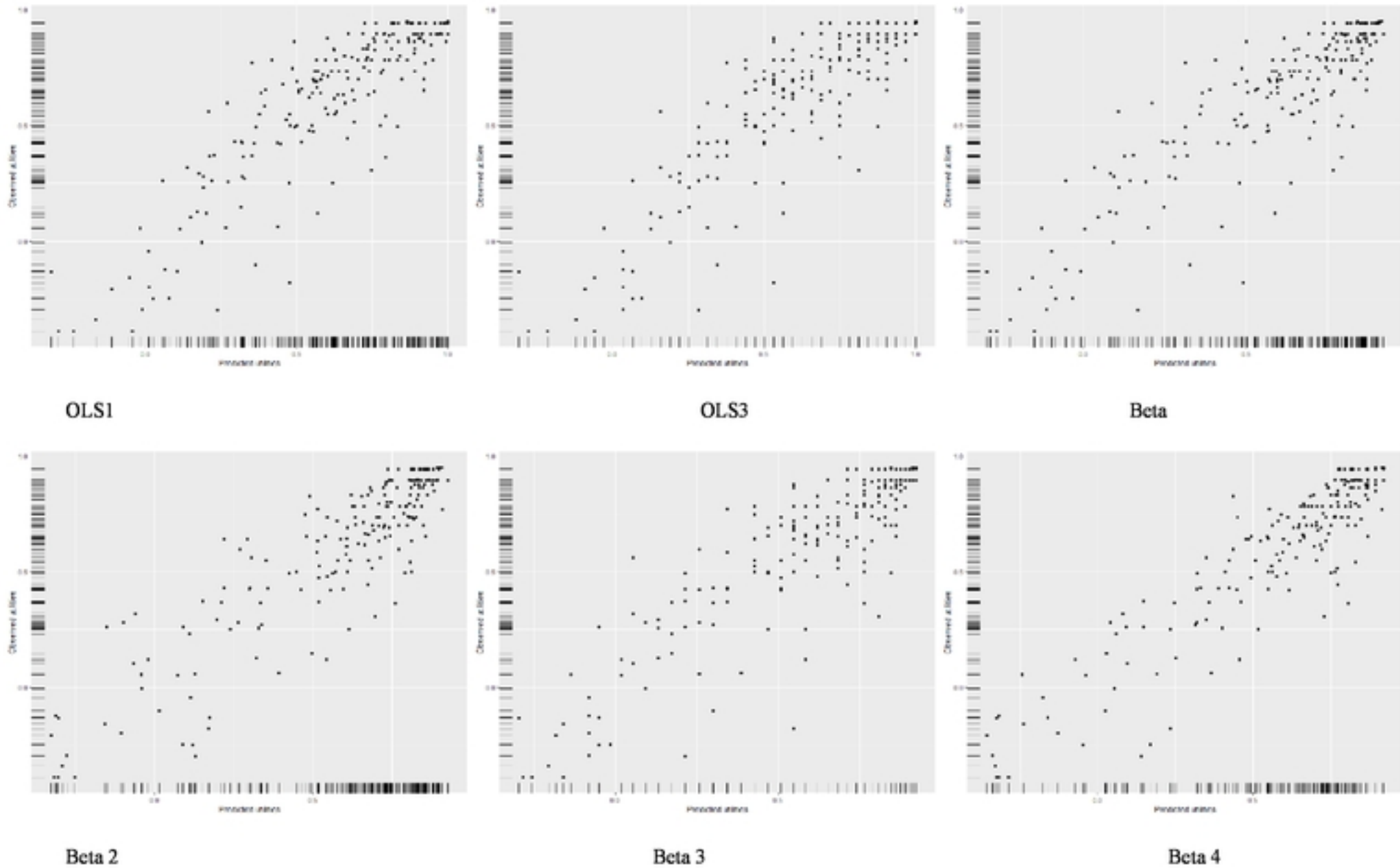
Fig.1 The scatter plots between observed and predicted utilities of selected models.
