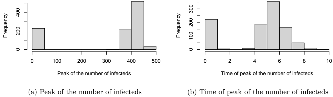
Figure 3: Results of 1000 simulated SIR epidemics
