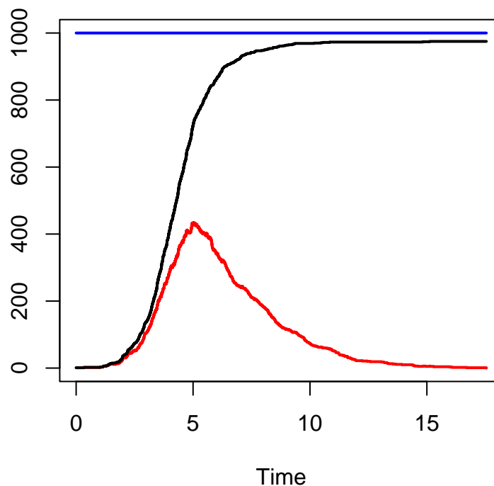
Figure 2: Stacked plot showing the number of susceptible, infected and recovered individuals over time from a stochastic SIR model.
