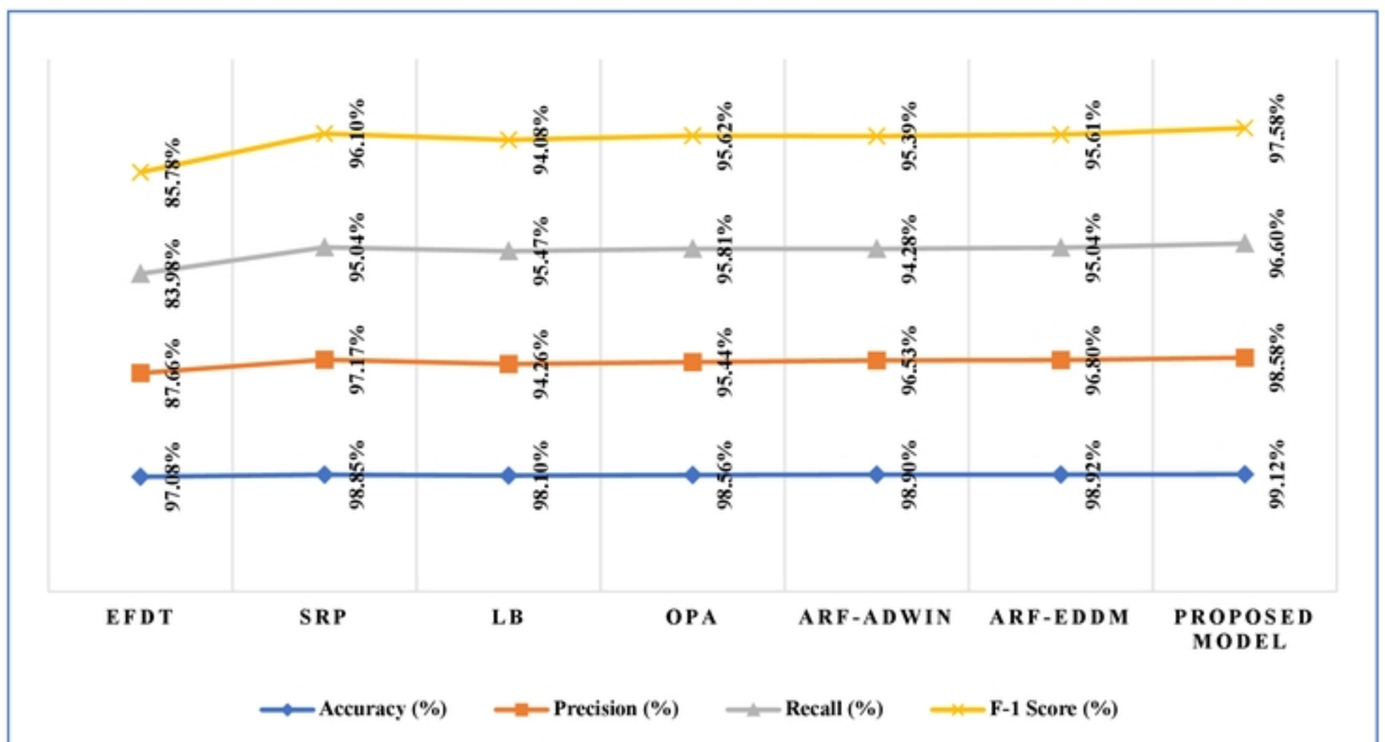
Figure 10. Proposed framework on CICIDS2017 dataset.
