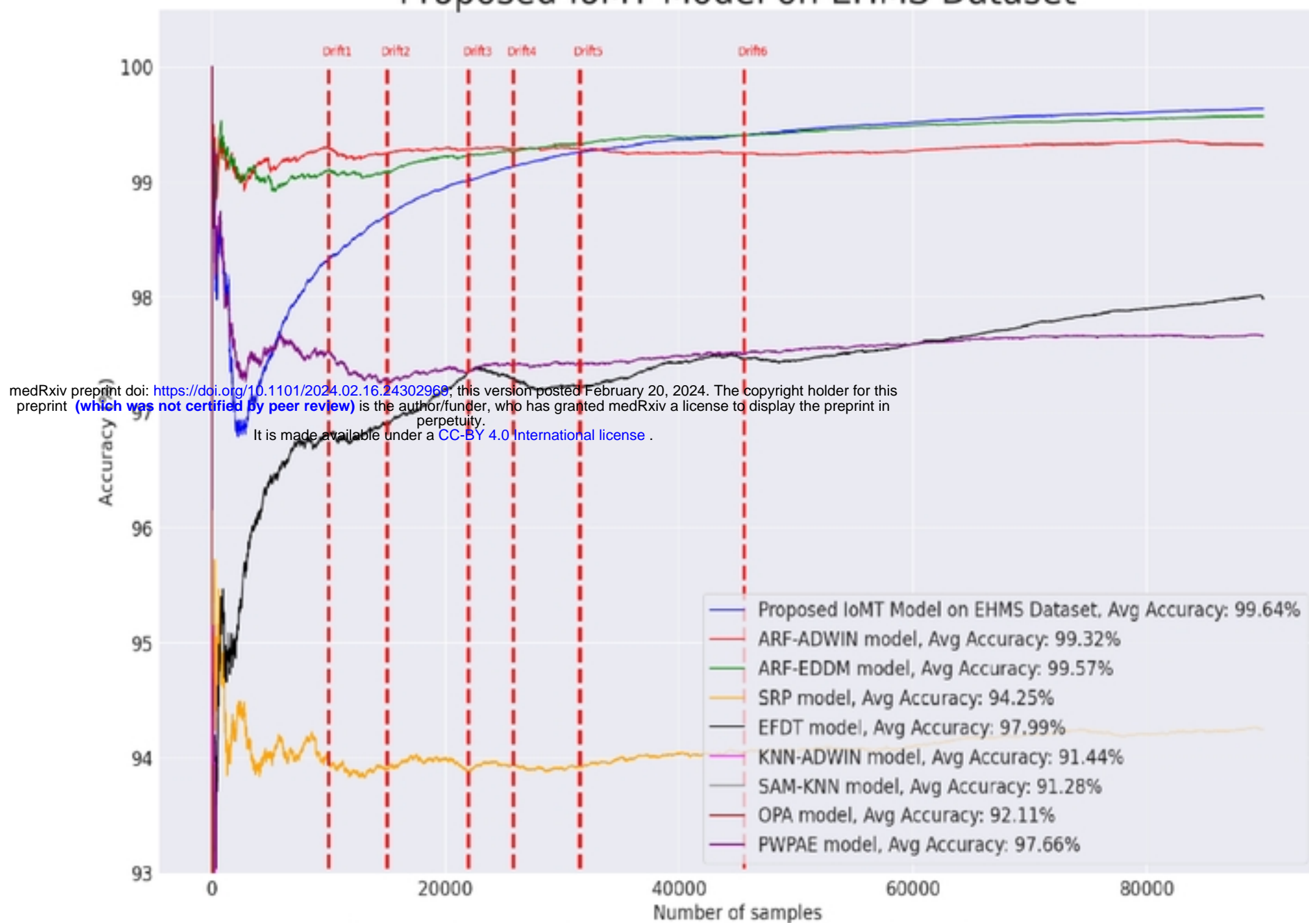
Figure 6. Proposed framework on WUSTL EHMS-IoMT dataset.
