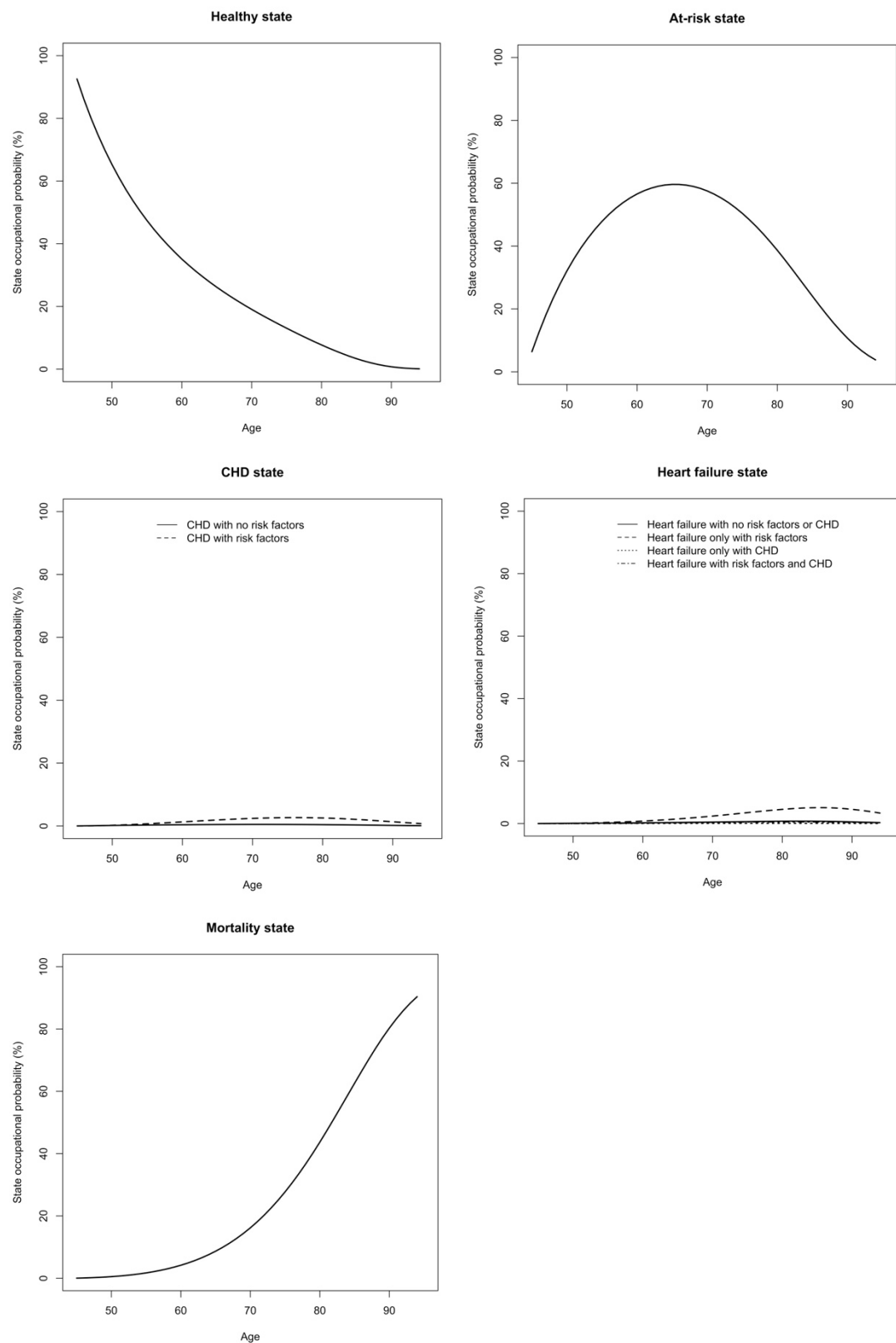
Figure 6. State occupational probabilities (%) starting from age 45 years estimated using the non-Markov framework in the Atherosclerosis Risk in Communities Study (ARIC) study.
