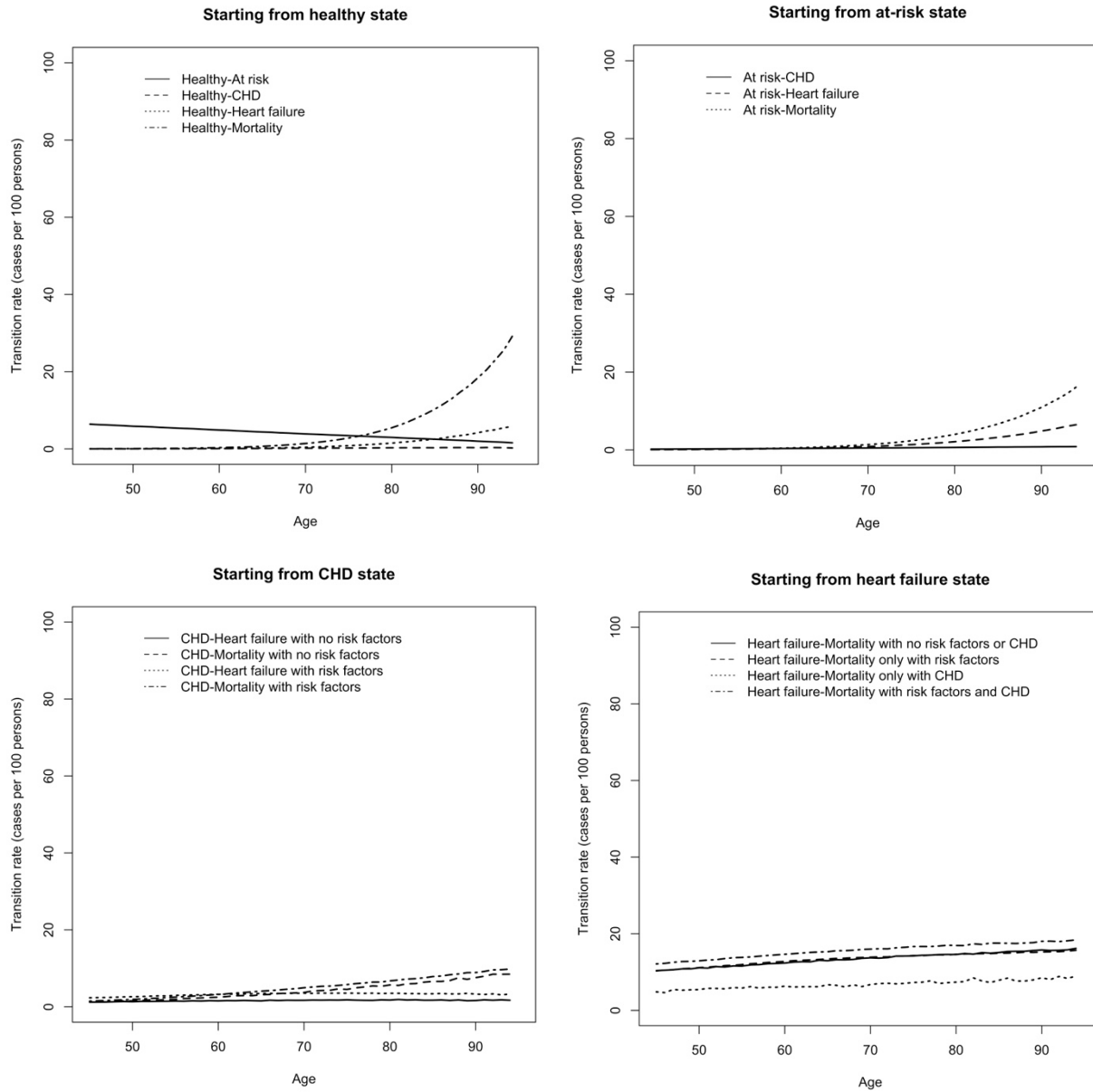
Figure 4. Age-specific transition rates (cases per 100 persons) from age 45 to 94 years estimated using the non-Markov framework in the Atherosclerosis Risk in Communities Study (ARIC) study.
