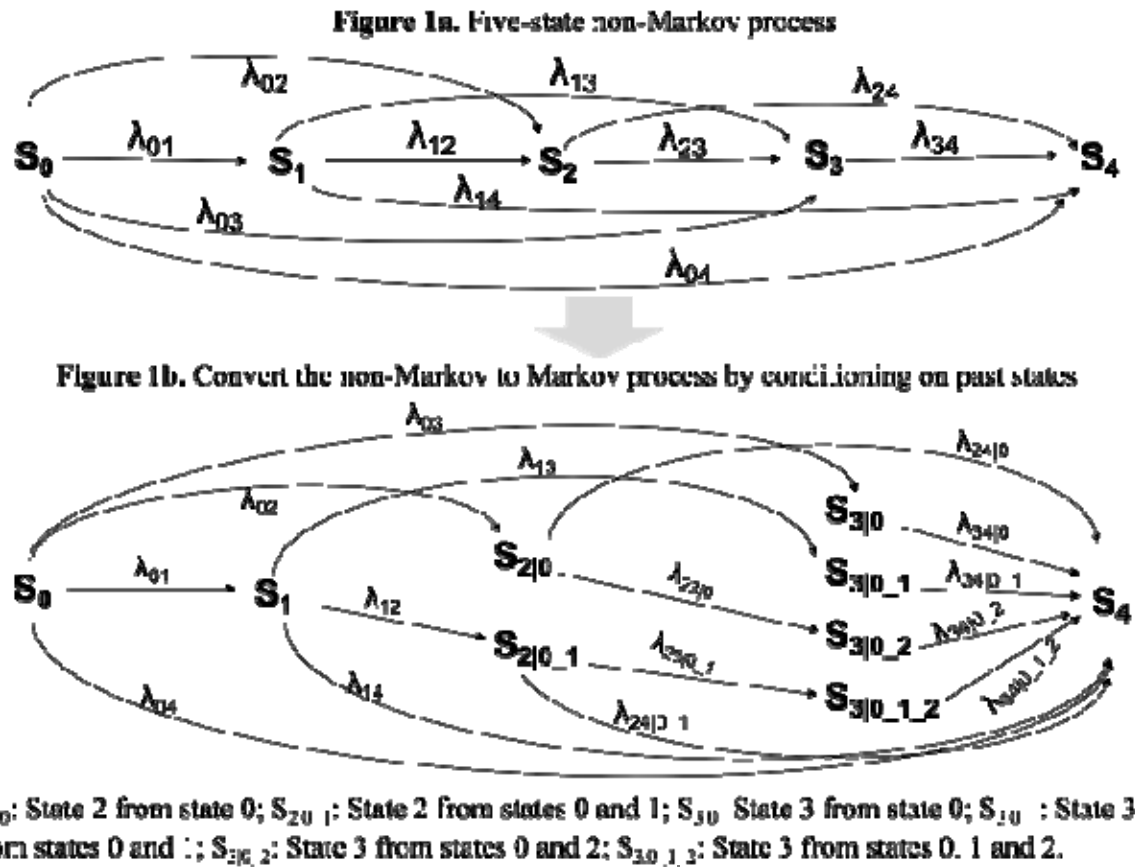
Figure 1. Convert non-Markov to Markov process by splitting disease states into substates.
