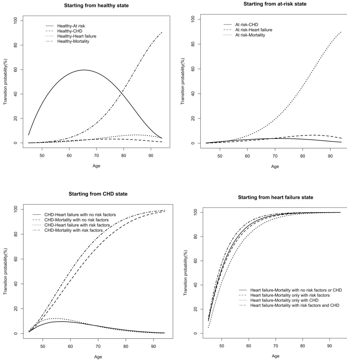
Figure 5. Transition probabilities (%) starting from age 45 years estimated using the non-Markov framework in the Atherosclerosis Risk in Communities Study (ARIC) study.
