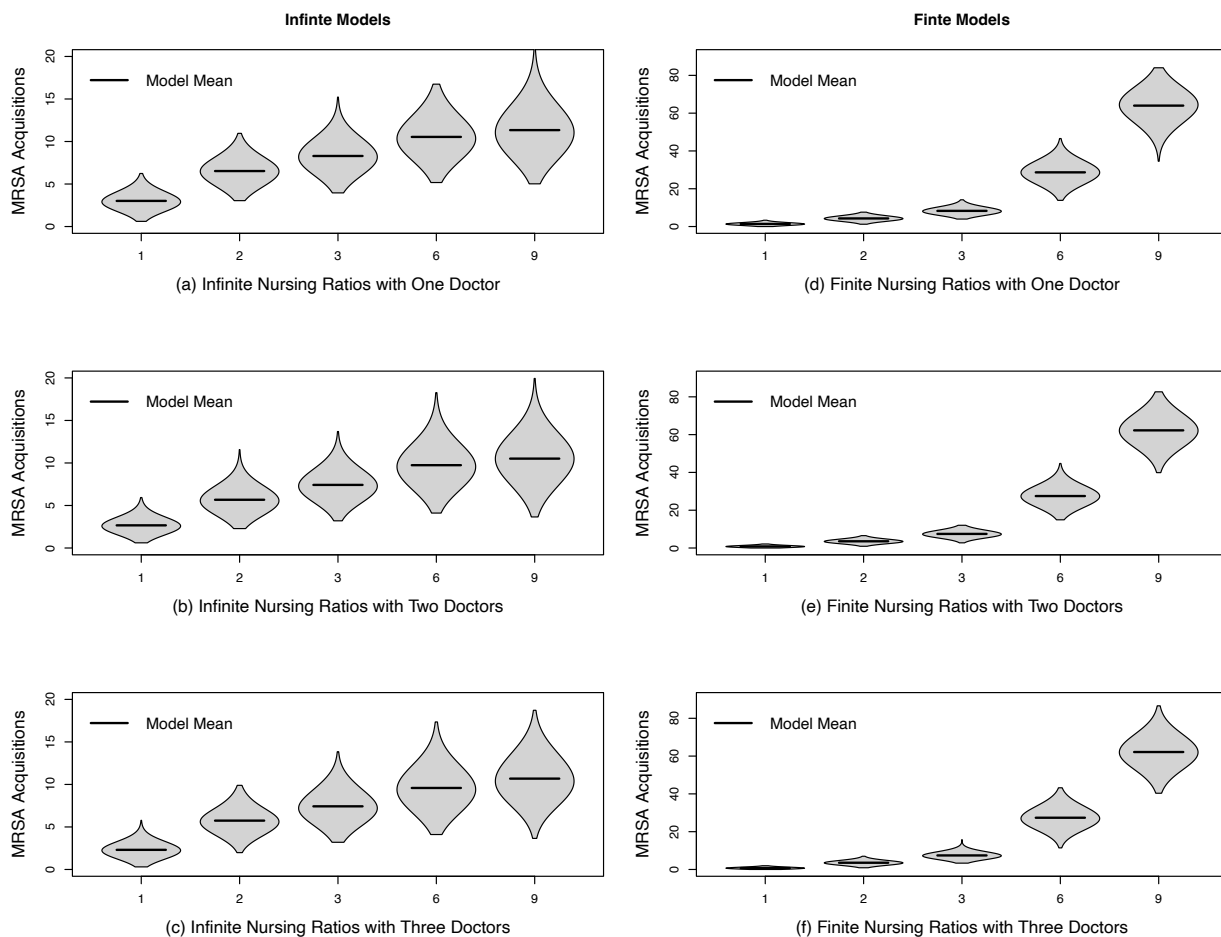
Figure 2. Distribution of cumulative MRSA acquisitions per 1000 patient-days in 1,000 simulated 18-bed ICUs under the different staffing ratios with both Finite and Infinite Task Scenarios
