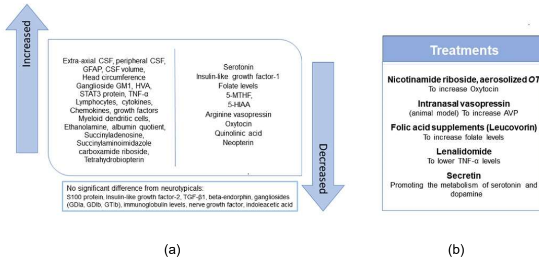
Fig 3: Summary of the CSF properties in ASD and the suggested treatments. Panel (a) summarizes the CSF properties that are increased, decreased, and not significantly different from neurotypicals. Panel (b) highlights the treatments, as mentioned in the literature for different abnormal physiological traits of CSF.
