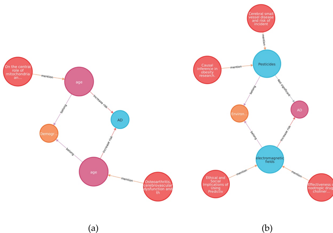
Figure 4. Demographic and environmental risk factors for AD: (a) illustrates that age is a risk factor of AD, and (b) illustrates that exposure to pesticide does not have significant effect on AD.
