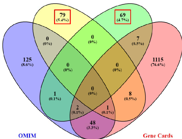
Figure 3: Venn diagram of the differentially expressed genes (DEGs).
