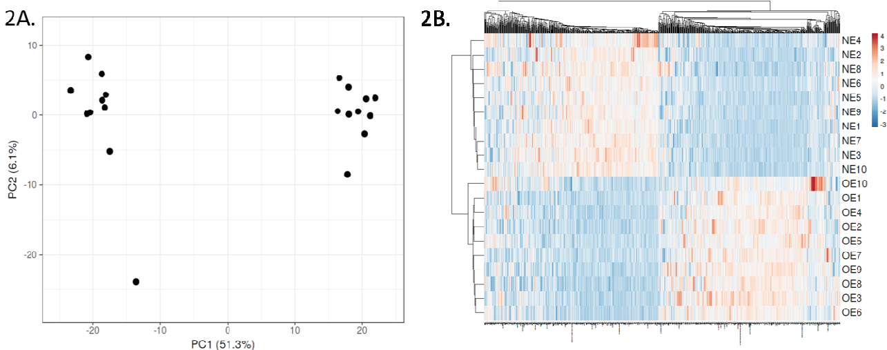
Figure 2: Heat map of DEG's. Blue to orange gradation is for small to large changes in gene expression values.
