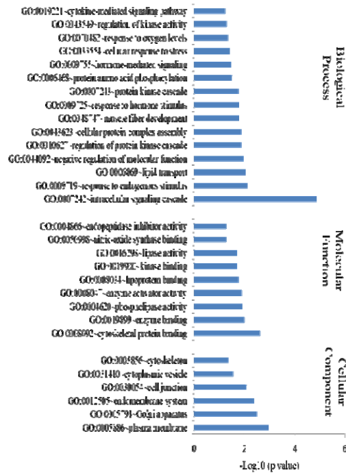
117 Figure 5: Gene Ontology (GO) enrichment analysis for up-regulated (5A) and down-regulated 118 DEG's (5B), and KEGG pathway enrichment for DEG's (5C).
