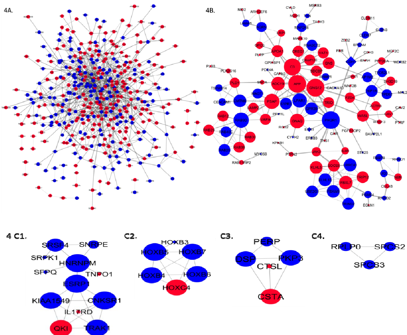
110 111 Figure 4: (A and B) Protein-protein interaction (PPI) of DEG's. C1, C2, C3 and C4 are four sub- 112 networks of DEG's: C1; sub-network 1, C2; sub-network 2, C3; sub-network 3, C4; sub-network 4. 113 Red-circle for up and blue-circle for down-regulated genes respectively. Blue diamond for similar 114 related genes and lines shows the correlation between genes, where thickness of lines (edges), is 115 proportional to the combined scores.
