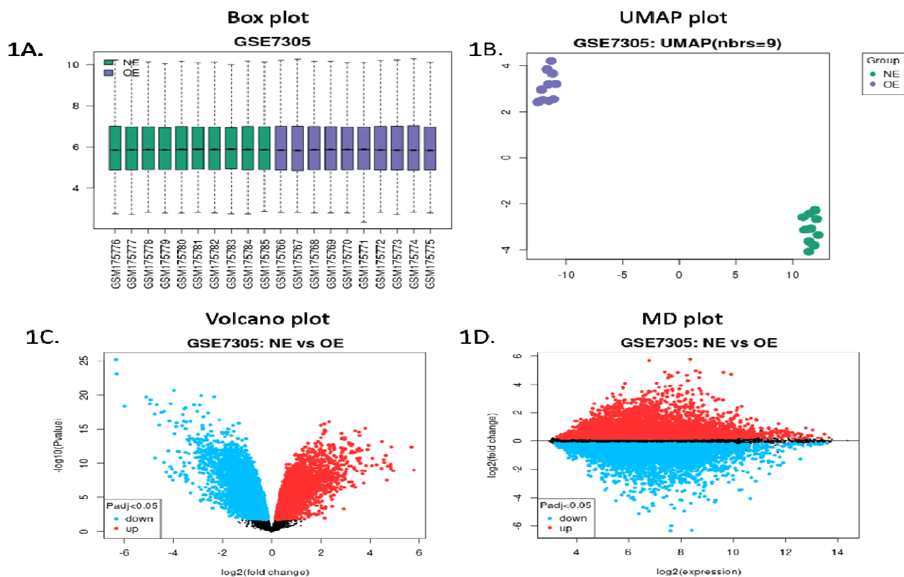
Figure 1: Data normalization and DEG's visualization via Box plot (A), UMAP plot (B), Volcano plot (C) and MD plot (D).
