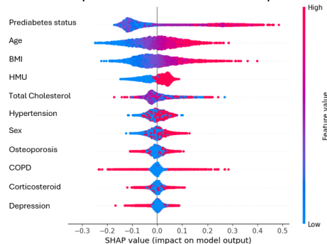
Fig. 2: SHAP scatter plot for prediabetes prediction DNN features.
