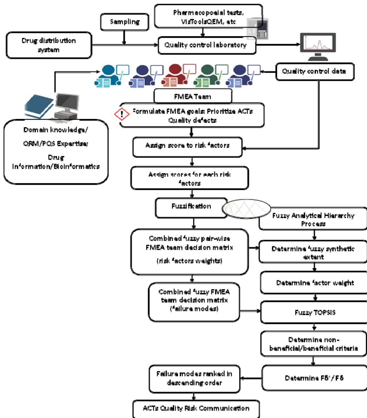
6 Figure 2: Systematic methodology for a hybrid fuzzy analytical hierarchy process and fuzzy 7 TOPSIS in failure mode effect analysis of fixed-dose artemether-lumefantrine tablets. 8 VisToolsQEM: Visual Tool for Quality Evaluation of Medicines, FMEA: Failure Mode Effect 9 Analysis, PQS: Pharmaceutical Quality Systems, QRM: Quality Risk Management, TOPSIS:
