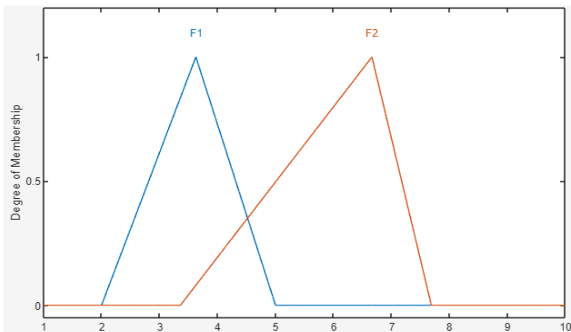
Figure 7: Comparison of fuzzy synthetic extents.
