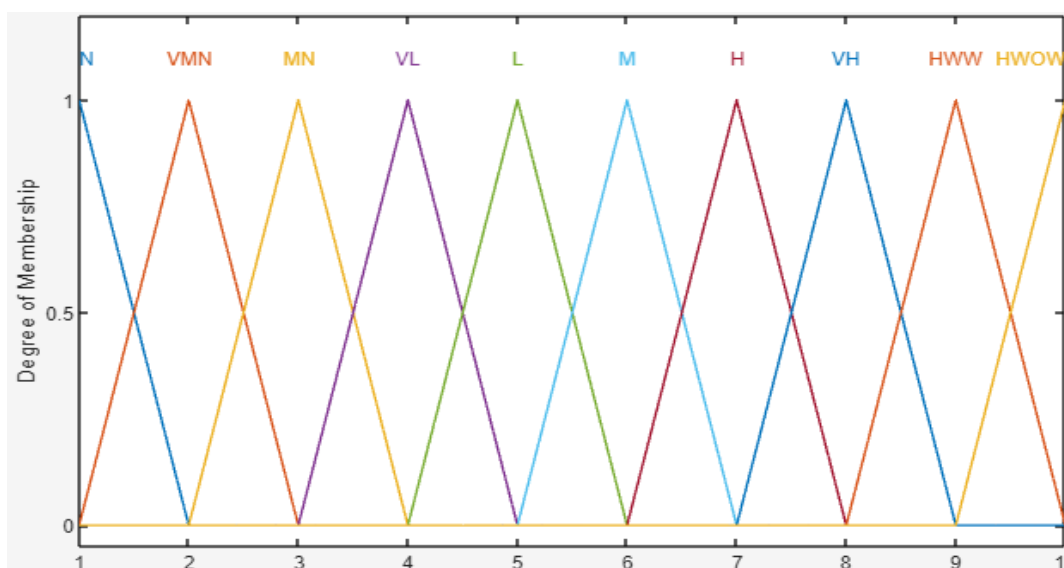
Figure 5: Membership functions for severity linguistic terms. N: None, VMN: Very minor, MN: Minor, VL: Very Low, L: Low, M: Moderate, H: High, VH; Very High, HWW: hazardous with warning; HWOW: Hazardous without warning.
