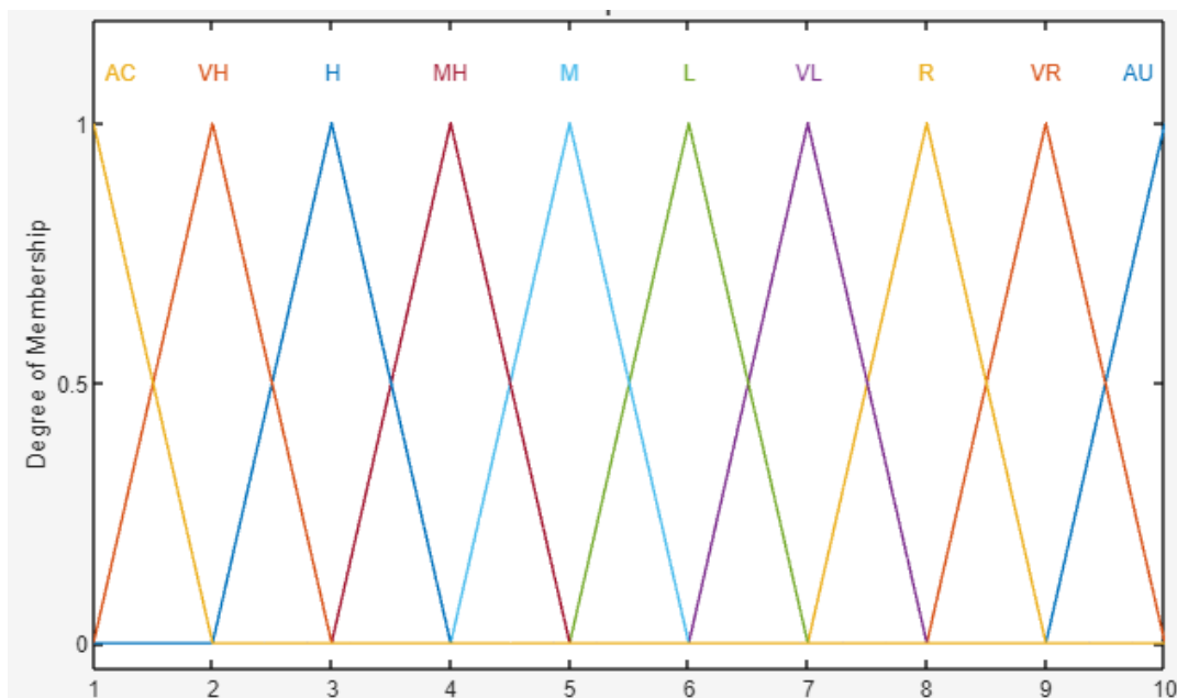
Figure 6: Membership functions for Detection linguistic terms. AC: Almost certain, Very Low, L: Low, M: Moderate, MH: Moderately high, H: High, VH; Very High, R: Remote, VR: Very remote, AU: Absolutely uncertain.
