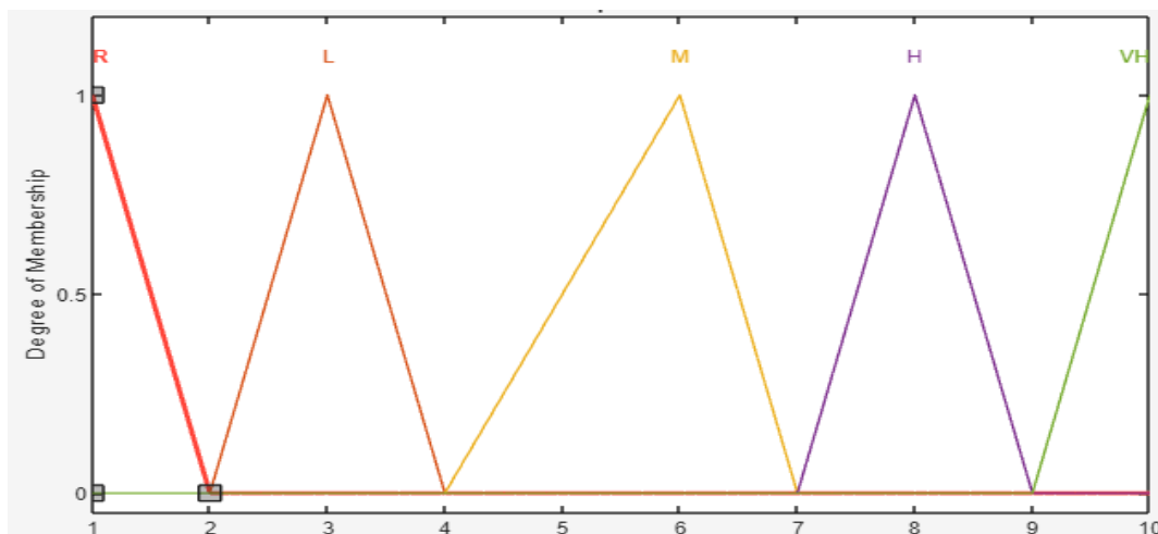
Figure 4: Membership function plot for Occurrence. R: Remote, L: Low, M: Moderate, H: High, VH; Very High.
