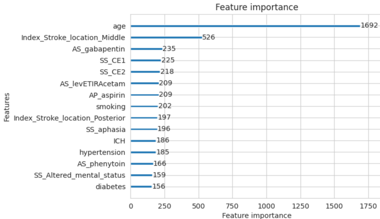
Figure 3: Top Important Features for LGBM Model.
