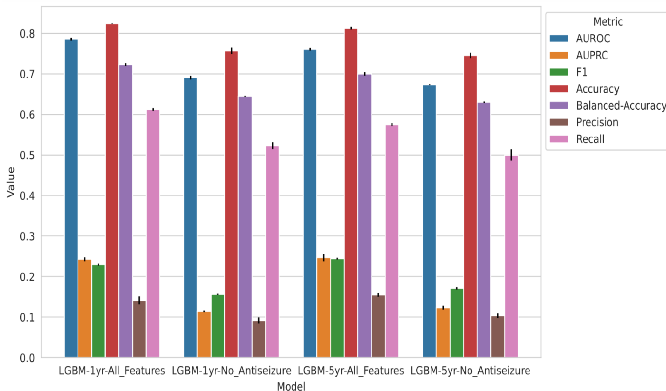
Figure 2: Visual Model Performance.
