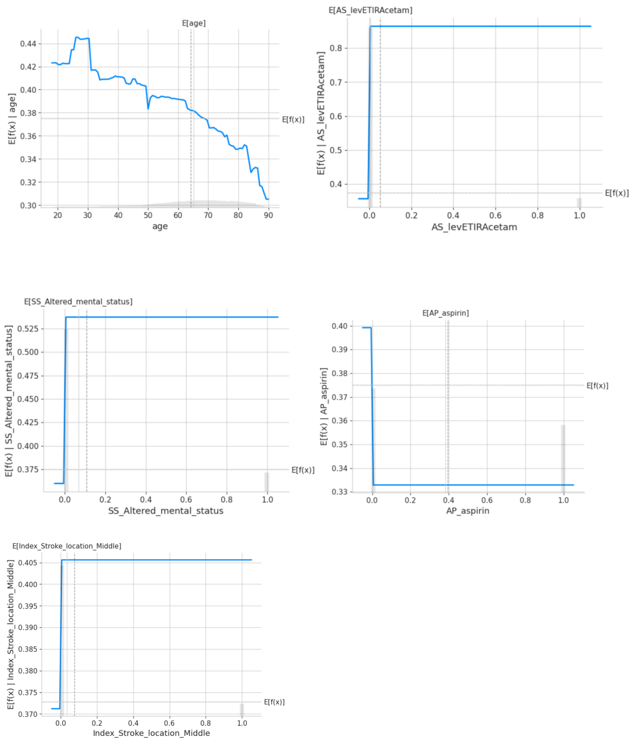
Figure 4: Partial dependence plots (PDP)
