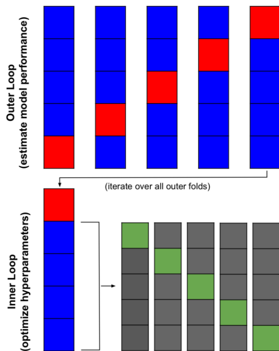
Figure 1: 5-fold Nested Cross Validation.
