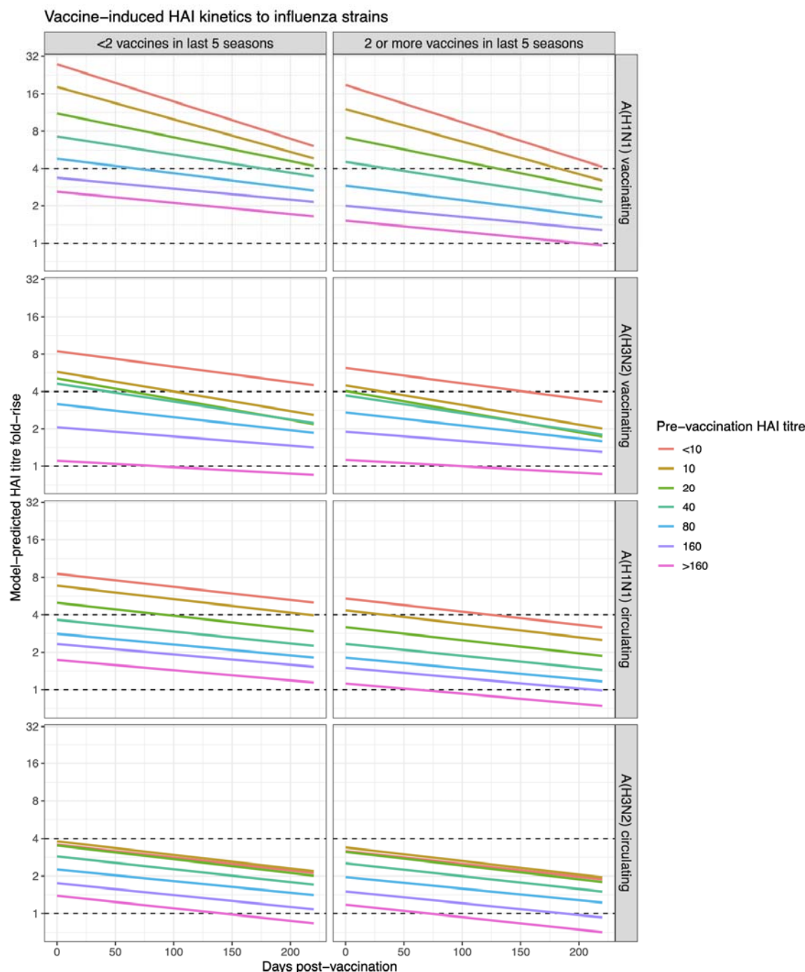
Figure 2. Expectation of post-vaccination kinetics from marginal posterior distributions of latent parameters. The mean post-vaccination HAI boosting (fold-rise) trajectories to virus strains stratified by pre-vaccination HAI titre and vaccination history (infrequently vaccinated and frequently vaccinated).
