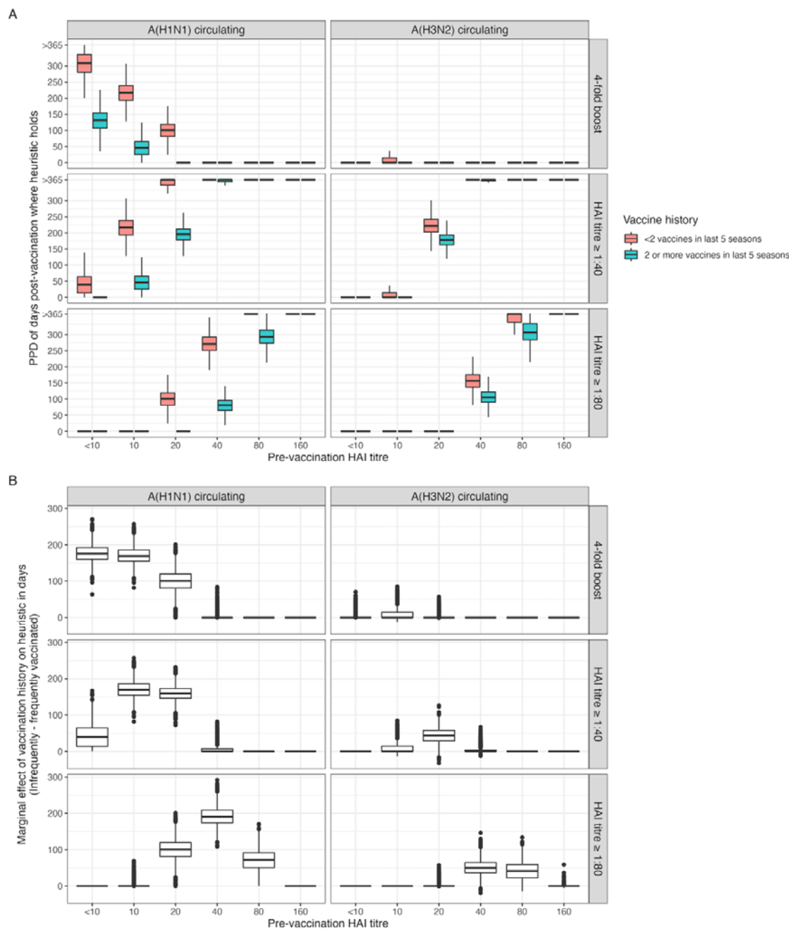
Figure 3. Post-vaccination duration of seroconversion and seroprotection from inferred statistical model. (A) Posterior predictive distribution (PPD) for the duration that titre rise is \geq 4 -fold and that HAI titre is \geq 1:40 and \geq 1:80 after vaccination stratified by vaccination history and pre-vaccination titre. (B) The PPD for the differences in days that titre rise \geq 4 -fold and that HAI titre is \geq 1:40 and \geq 1:80 between the two vaccine histories.
