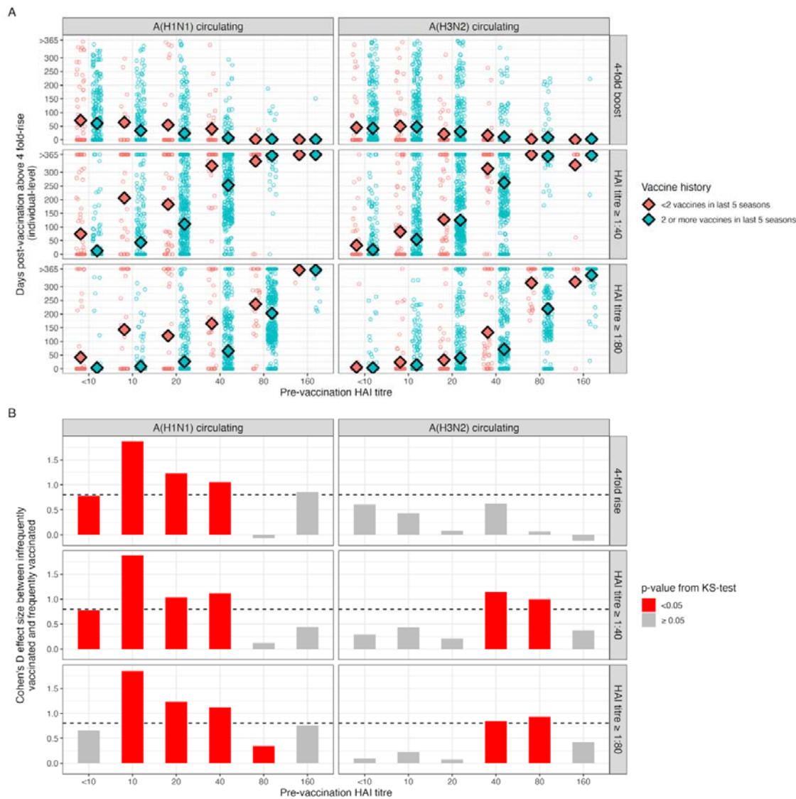
Figure 4. Post-vaccination duration of seroconversion and protection when considering outcome variability. (A) Individual-level estimates for the duration that titre rise is \geq 4 -fold and that HAI titre is \geq 1:40 and \geq 1:80 after vaccination stratified by vaccination history and pre-vaccination titre. Large diamond point marker individuals mean of sample. (B) Effect size from Cohen's D and the p-value from a Kolmogorov-Smirnov test to assess the significance of the difference between the two vaccine history levels for the duration post-vaccination above a threshold heuristic.
