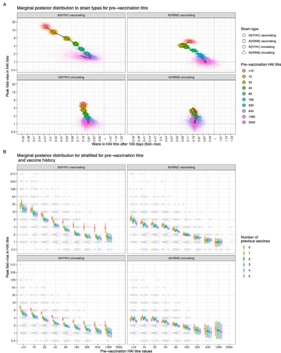
Figure 1. Bayesian marginal posterior distribution for covariates as a measure of inferential uncertainty. (A) The marginal posterior distributions of boosting and waning stratified by pre-vaccination HAI titre for the four virus strains. The point markers are the mean value of the
