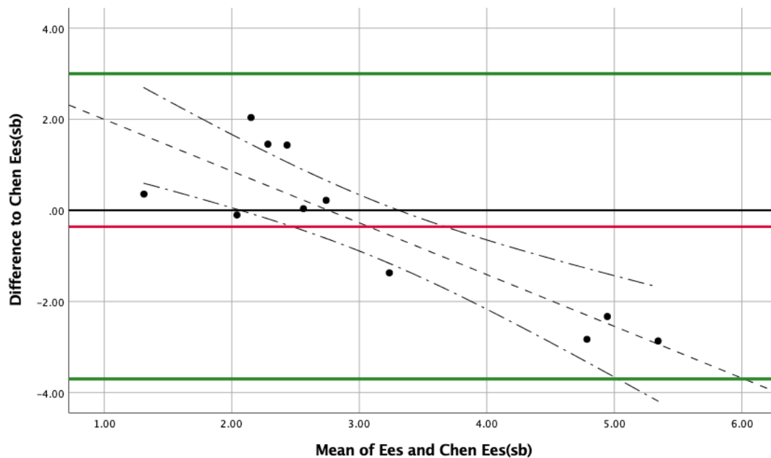
Figure 1: Bland-Altman plot - the agreement between Chen Ees(sb) and invasive Ees.
