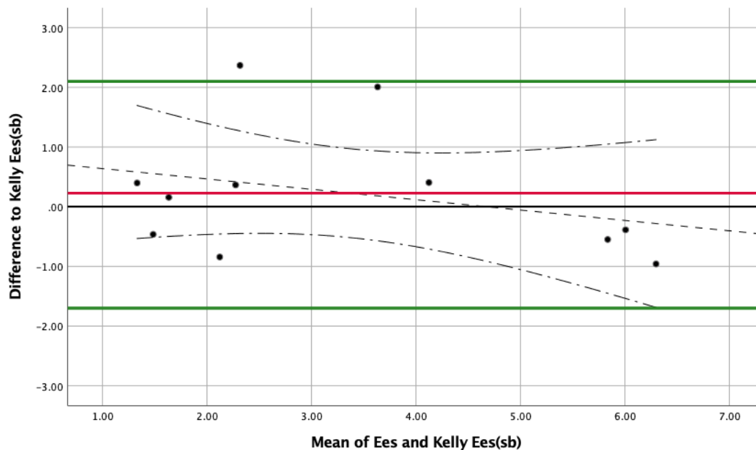
Figure 2: Bland-Altman plot - the agreement between Kelly Ees(sb) and invasive Ees.
