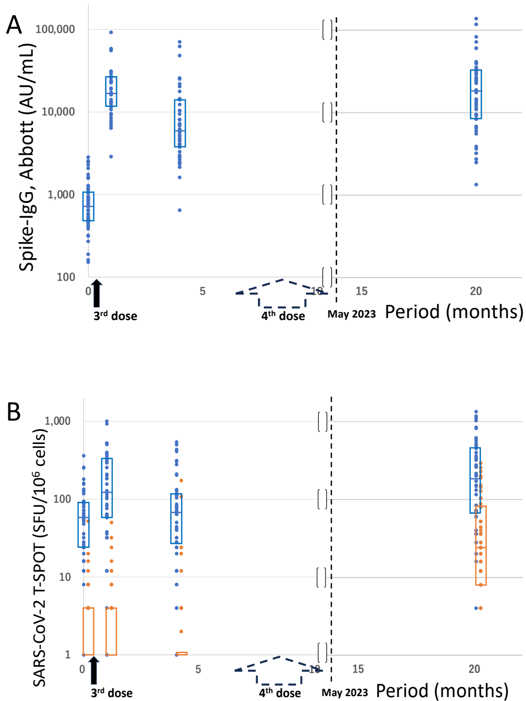
Figure: Time-elapsed values of Spike-IgG and those of T-SPOT for SARS-CoV-2.
