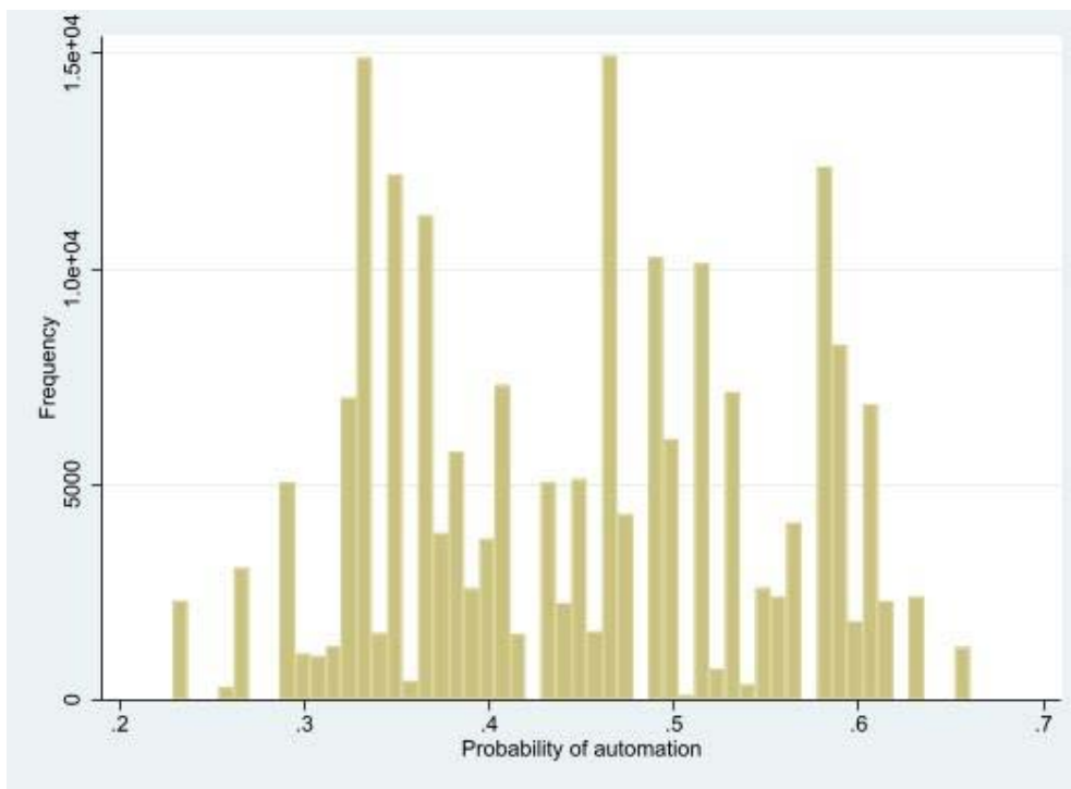
Figure A-1. The histogram of the probability of job automation for the entire sample.
