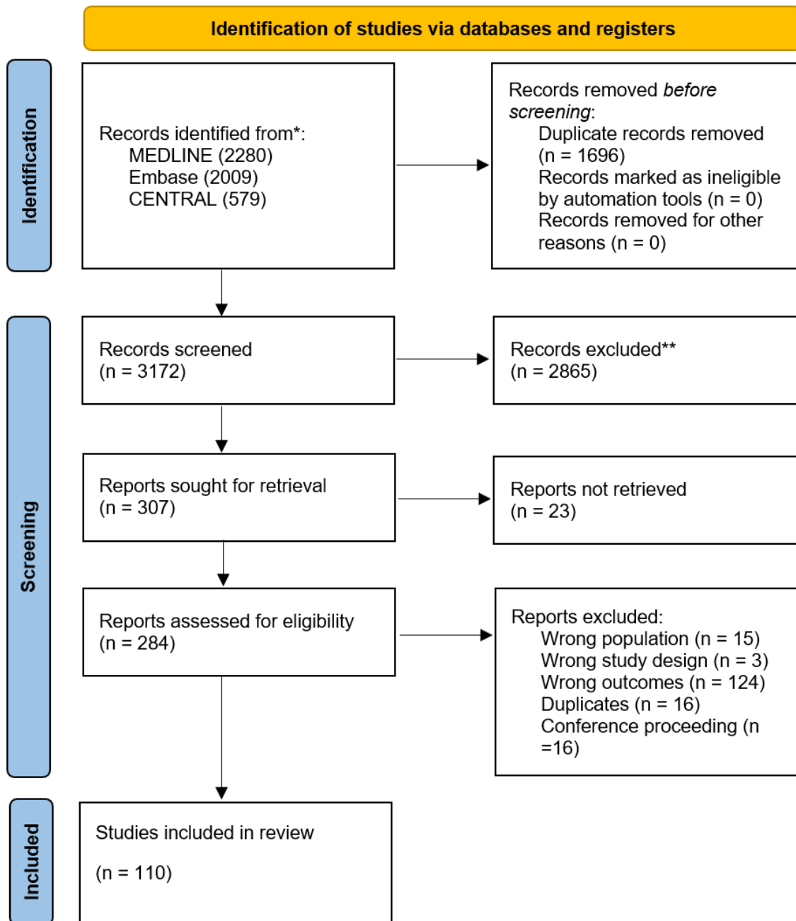
Figure 1. PRISMA flow diagram of screening process
