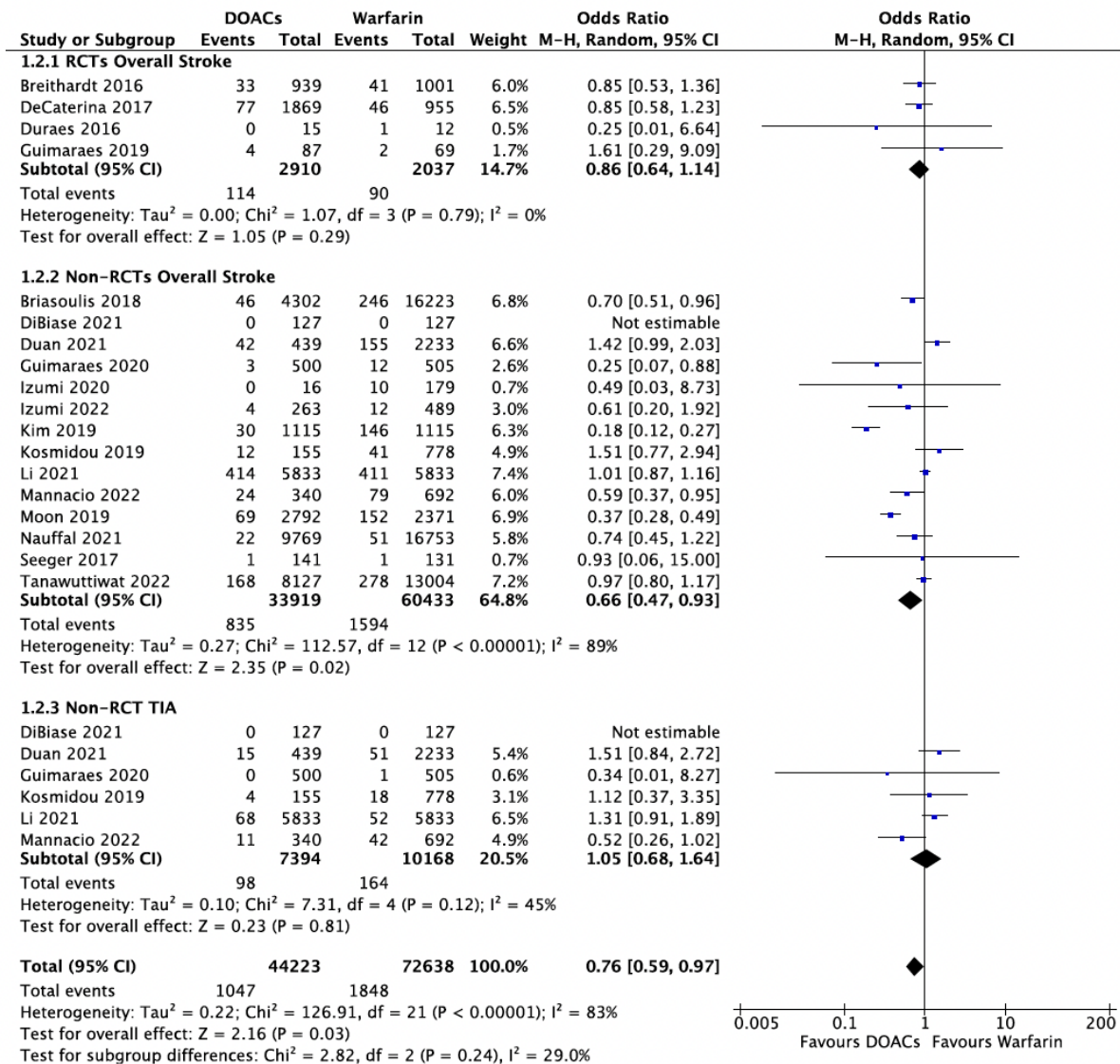
Figure 6. Association between stroke and TIA incidences with anticoagulation choice of DOAC versus warfarin in patients with concomitant atrial fibrillation and valve disease.
