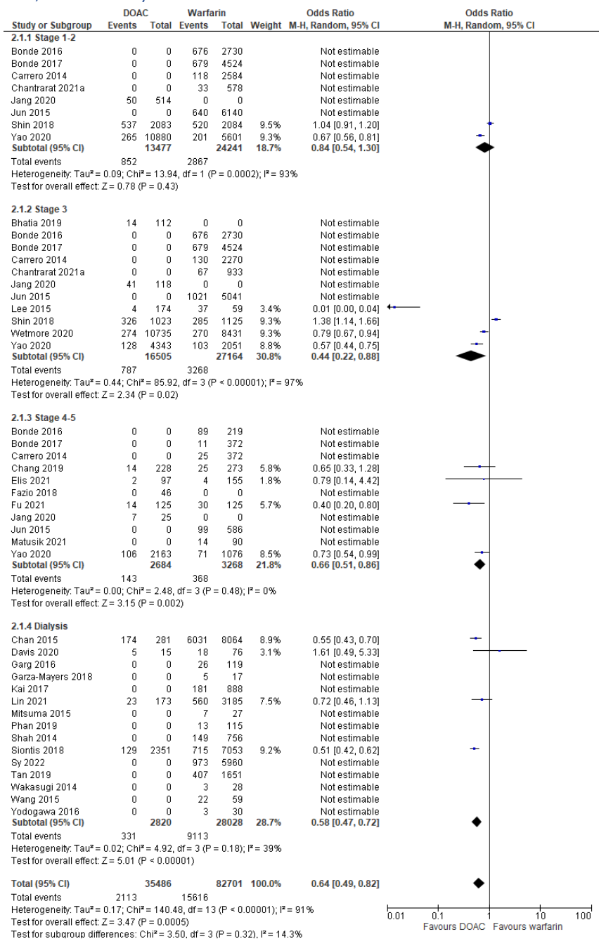
Figure 4. Association between number of bleeds and anticoagulation choice of DOAC versus warfarin in patients with concomitant atrial fibrillation and CKD of stages 1-2, stage 3, stage 4-5, or on dialysis.
