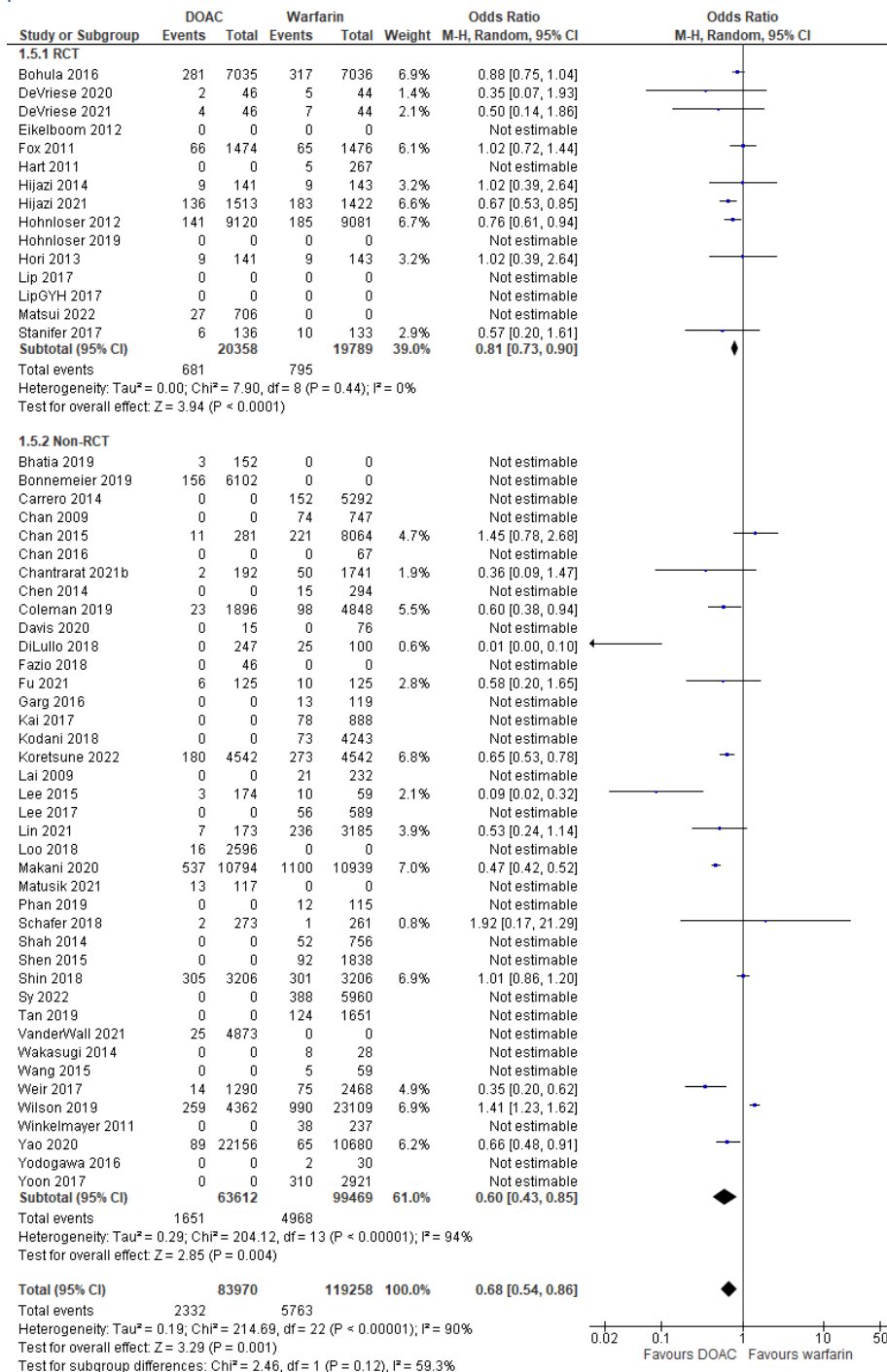
Figure 3. Association between incidence of strokes and anticoagulation choice of DOAC vs warfarin in patients with concomitant atrial fibrillation and CKD.
