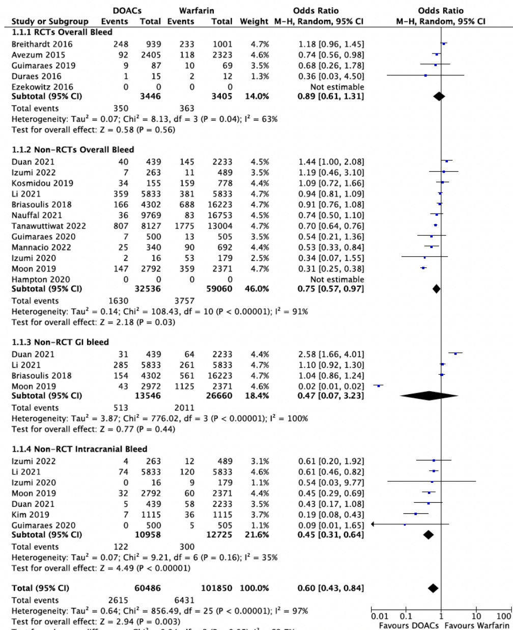
Figure 5. Bleeding outcomes with warfarin vs DOAC in patients with concomitant atrial fibrillation and valve disease.
