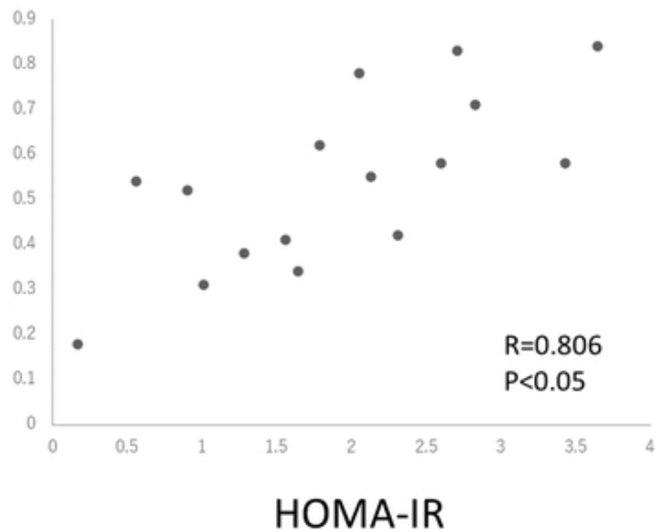
b. HOMA-IR vs mean total insulin dose/kg
