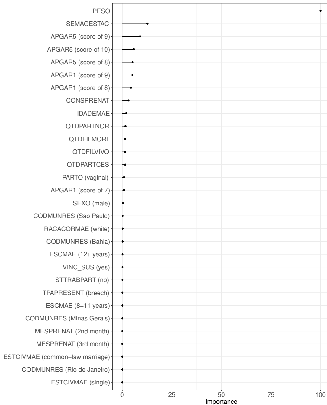
Figure 4: XGBoost feature importance.
