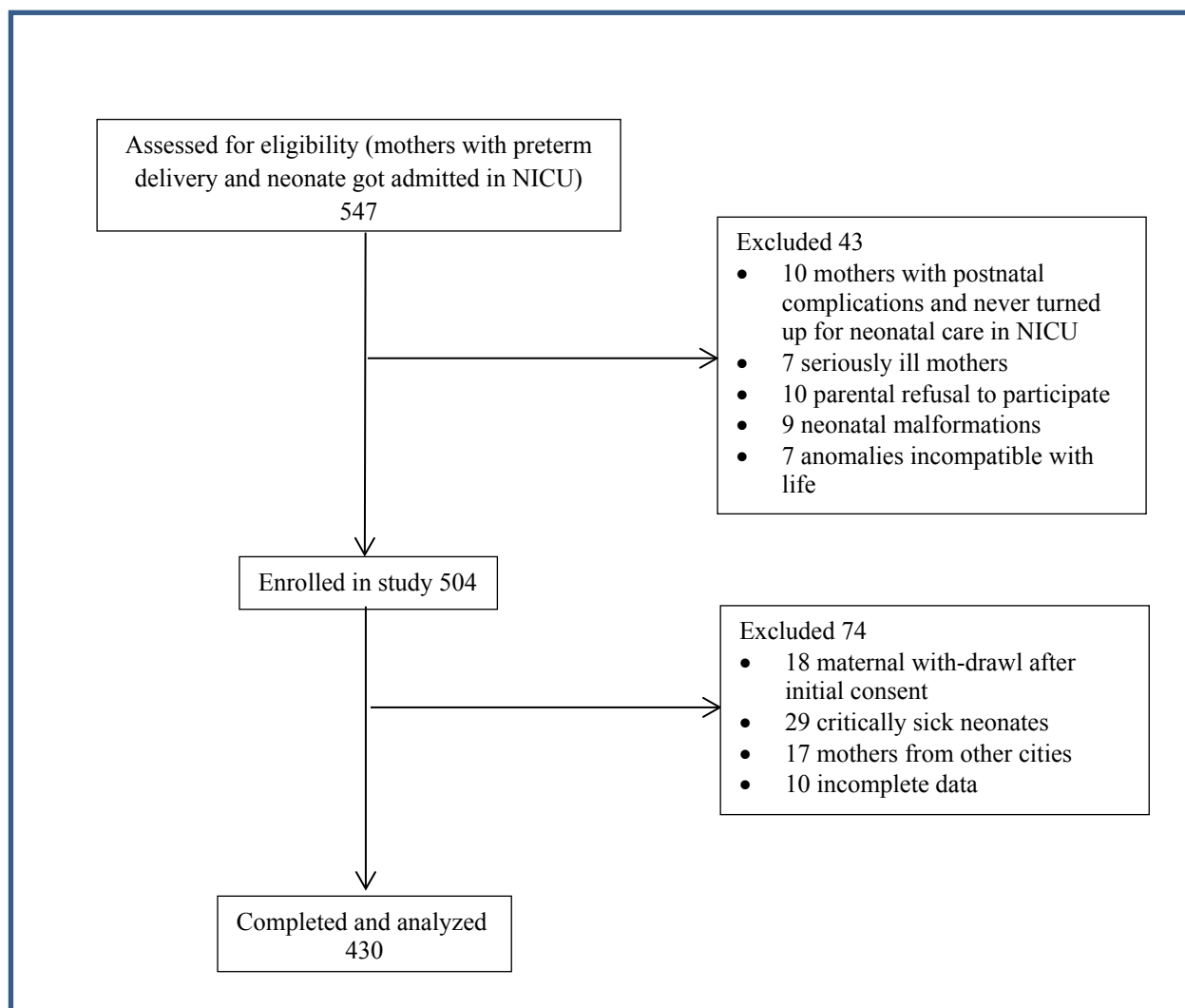
Figure 1: Consort diagram
