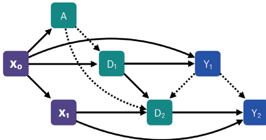
Figure 1: DAG representing the relationships among the exposures ( A , D_1 , D_2 ), the outcomes ( Y_1 , Y_2 ), and the covariates ( X_0 , X_1 ). Dashed lines indicate deterministic relationships.
