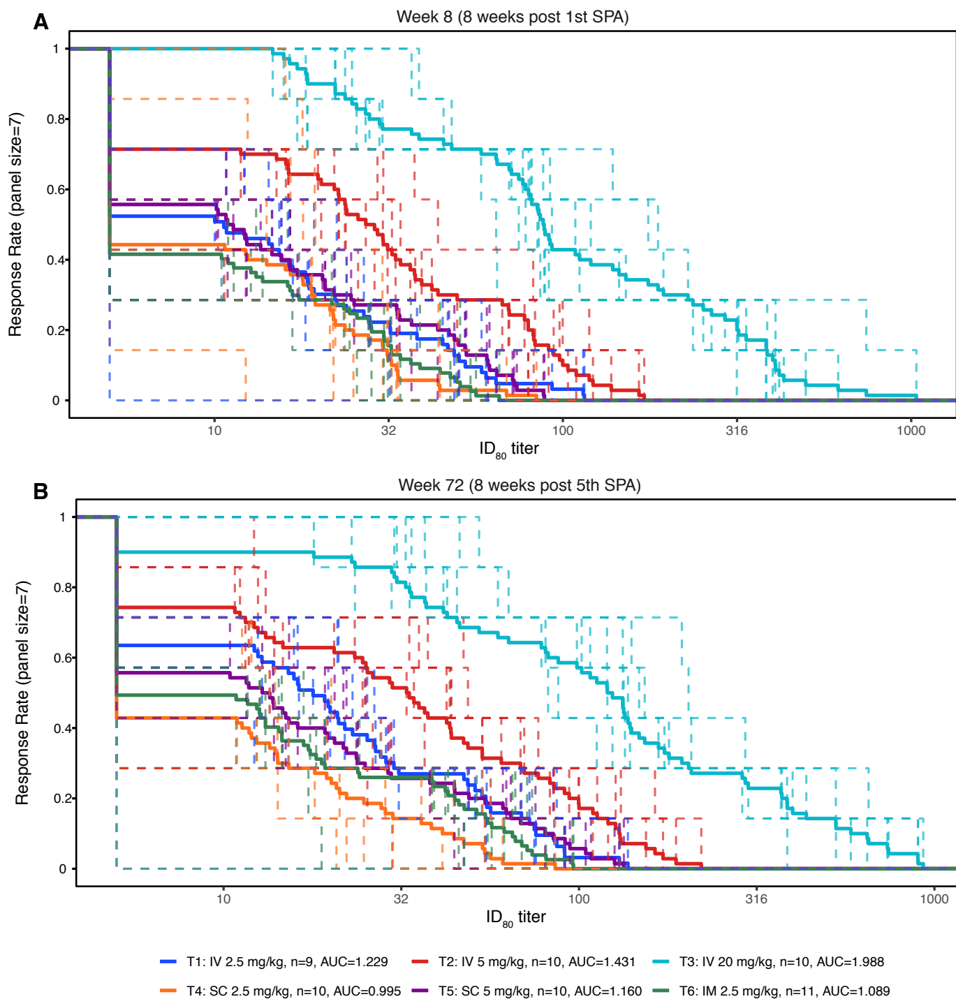
Figure 7. Magnitude-breadth curves for participant serum following VRC07-523LS administration against a panel of HIV-1 isolates collected from incident HIV-1 acquisition events in placebo recipients in the AMP trials. ID 80 titre is shown at Week 8 ( A ) and Week 72 ( B ).
