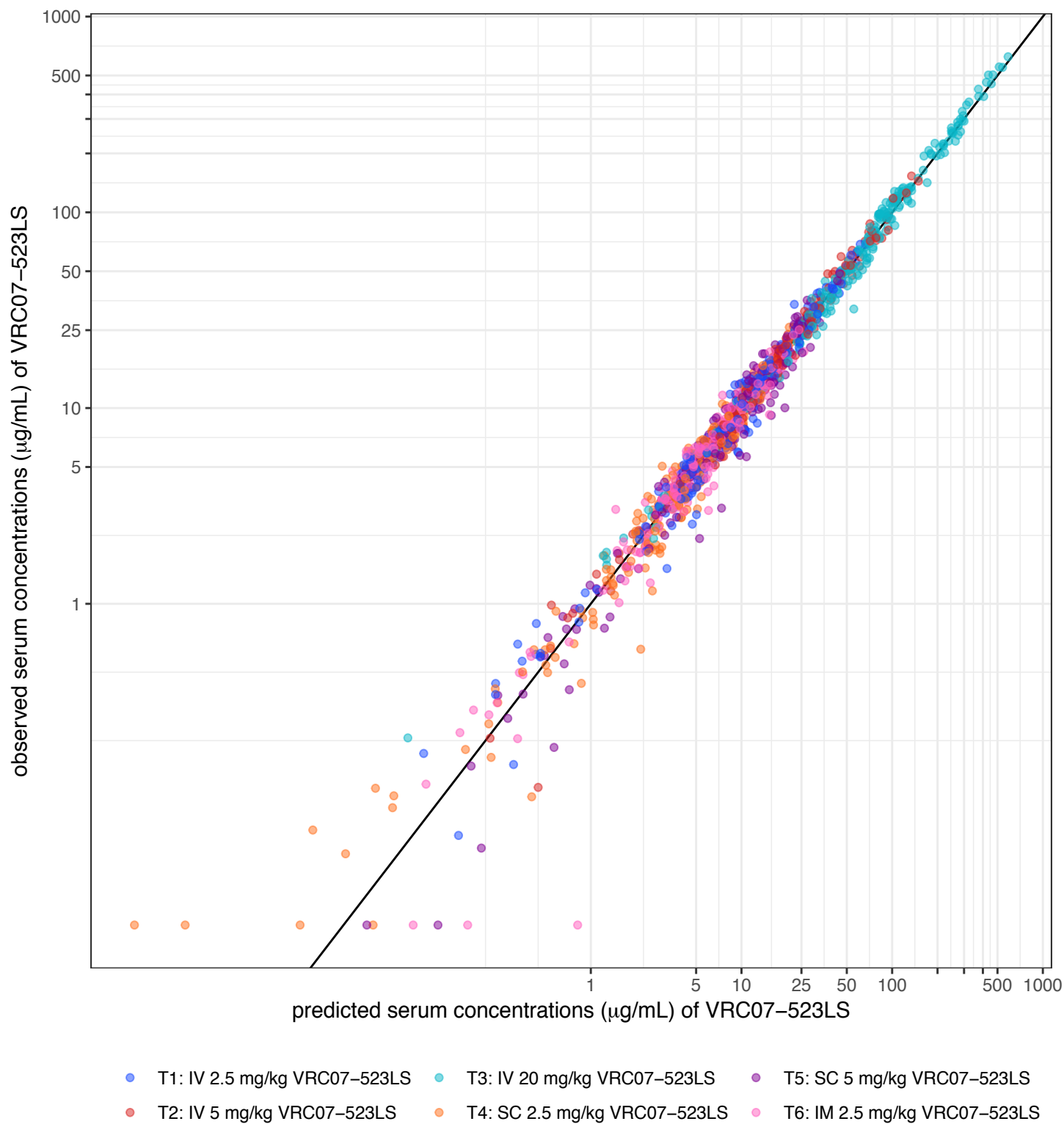
Figure 5. Measured serum concentrations of VRC07-523LS vs concentrations predicted by a two-compartment pharmacokinetic model.
