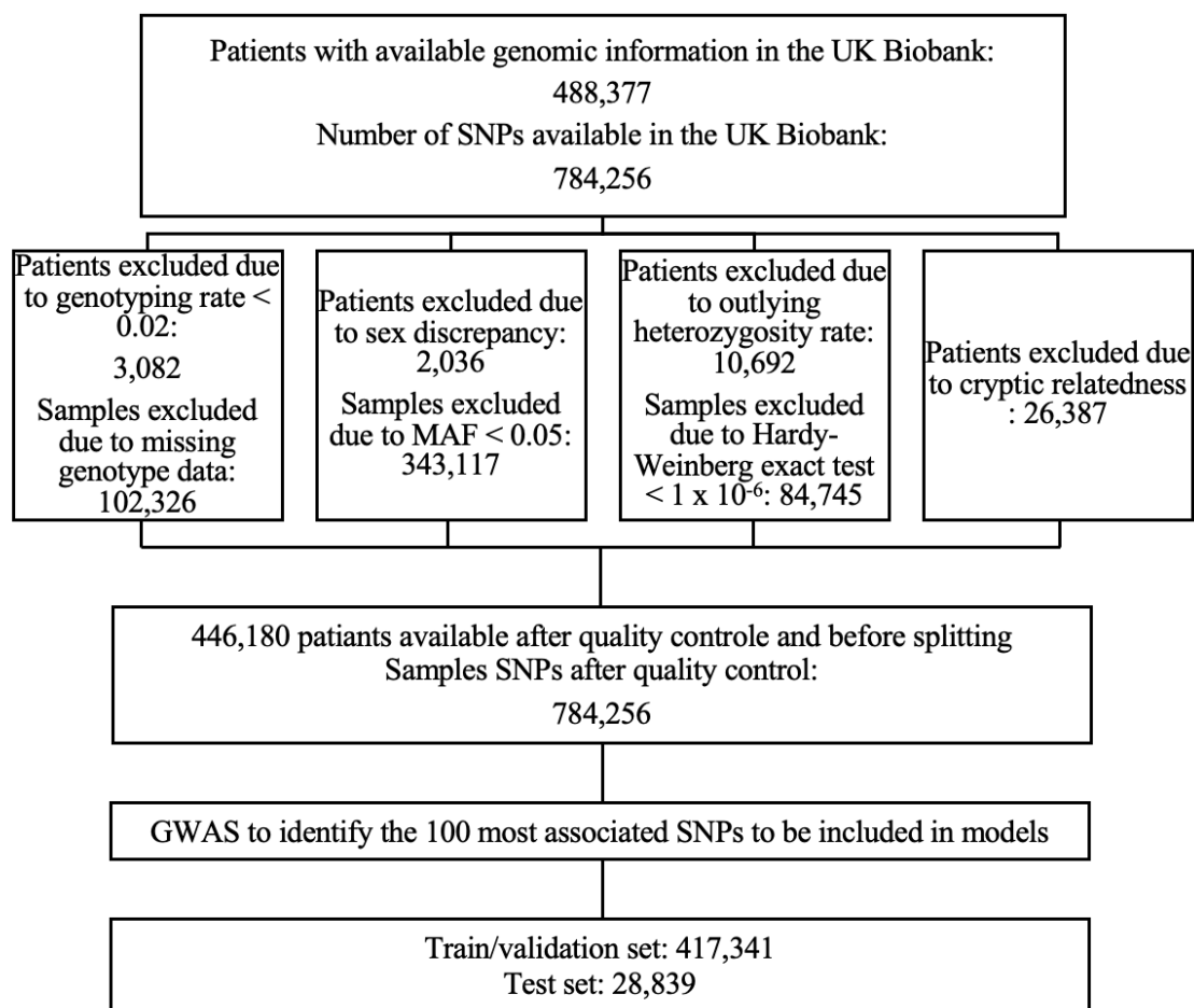
620 Figure 4: Selection and quality control steps of individuals and SNPs in the UKB
