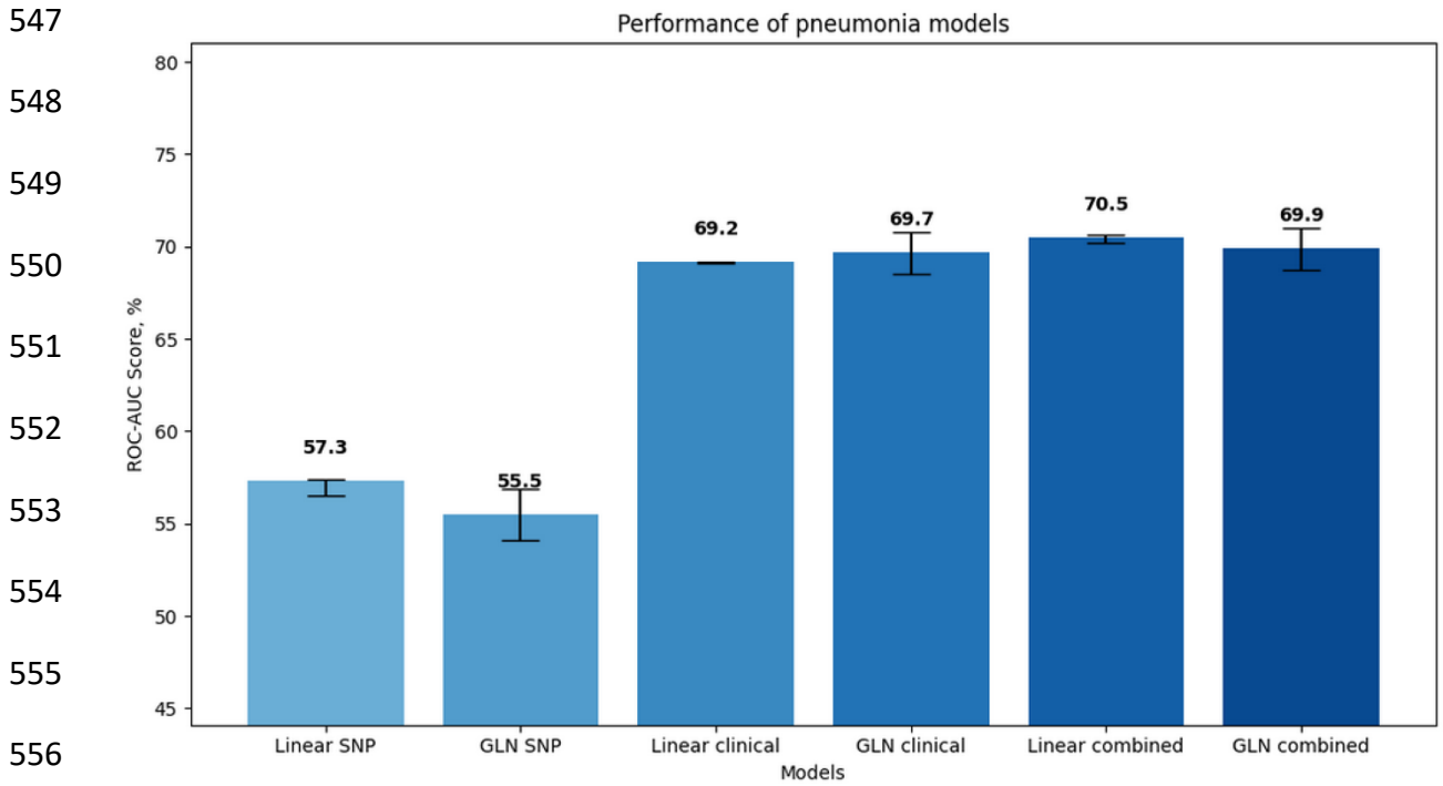
546 Figure 3C: Bar plot of ROC-AUCs of all pneumonia models
