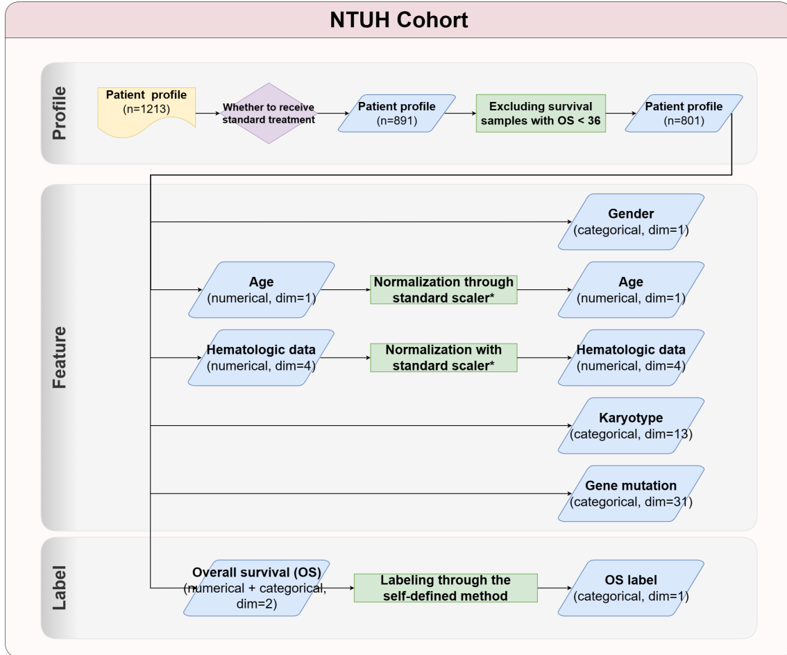
Figure 1. Feature selection and data preprocessing on the NTUH cohort. *Standard scaler is a normalization method in scikit-learn. 13
