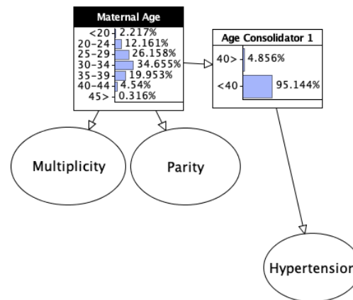
Figure 6: Maternal Age substructure showing hidden Age Consolidator node
