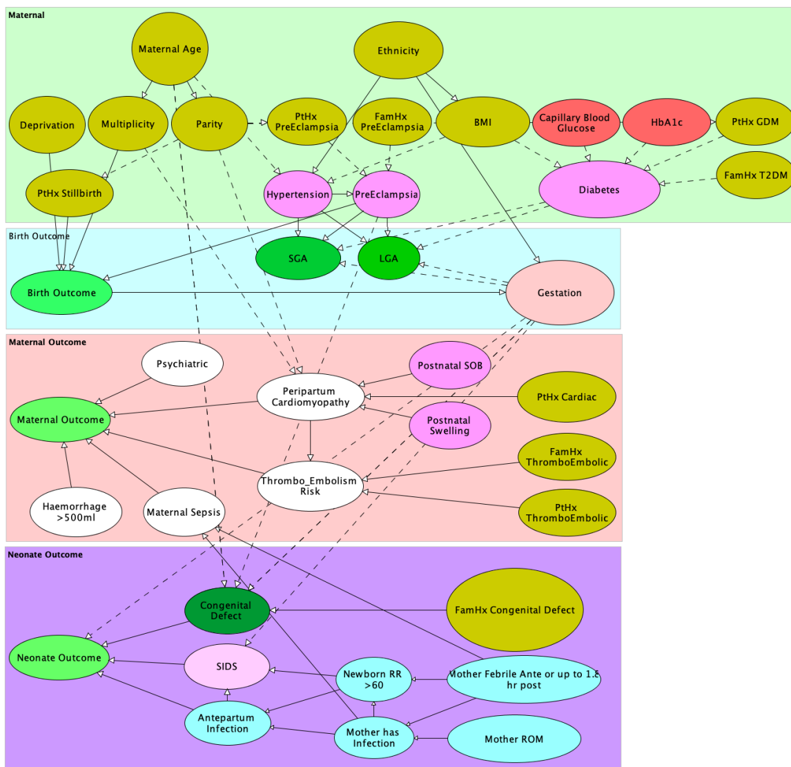
Figure 4: BN model for pregnancy outcomes
