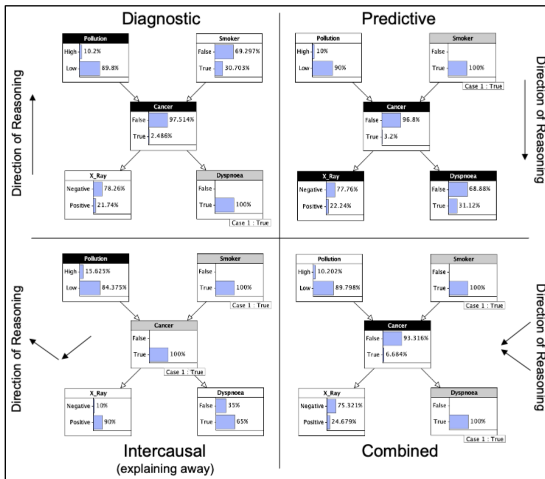
Figure 1: Types of reasoning
