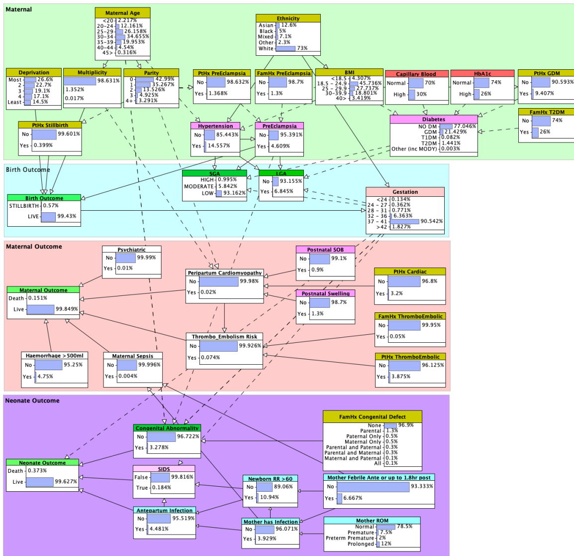
Figure 5: BN model showing background priors
