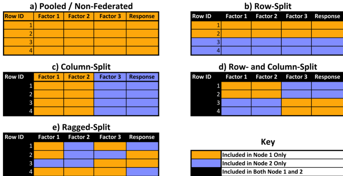
Figure 1. Approaches to splitting data across federated models
