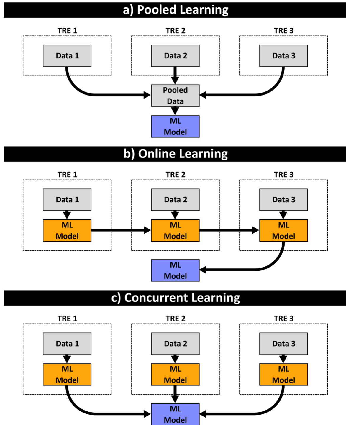
Figure 3. Schematic of the learning methods utilised for federated machine learning.
