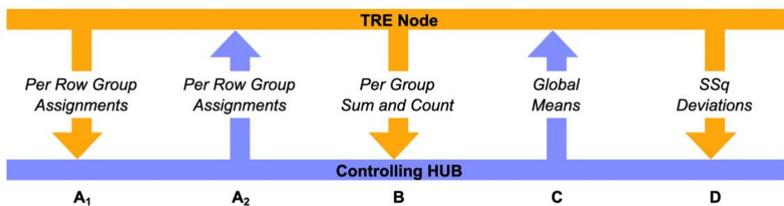
Figure 2. Data communications in a federated ANOVA environment
