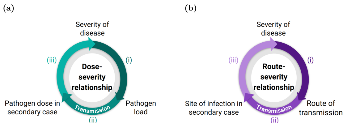
Fig. 1. Cycle diagrams depicting two symptom propagation mechanisms: dose-severity relationships and route-severity relationships. (a) A dose-severity relationship arises when (i) an individual's disease severity determines their pathogen load; (ii) pathogen load affects the infectious dose with which they infect others; (iii) this infectious dose then determines the disease severity in the secondary case. (b) A route-severity relationship arises when (i) an individual's disease severity determines the transmission route through which they infect others; (ii) the transmission route then determines the site of infection in the secondary case; (iii) the site of infection then affects their disease severity.
