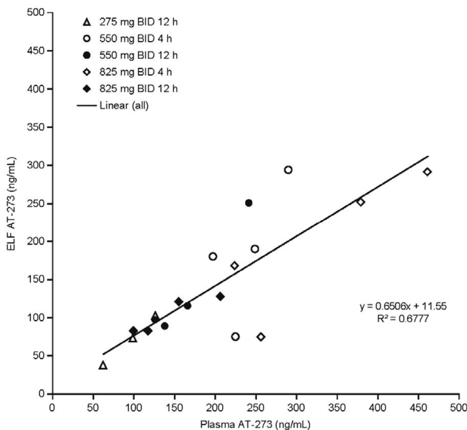
202 Figure 3. Correlation between plasma and ELF AT-273 levels.
