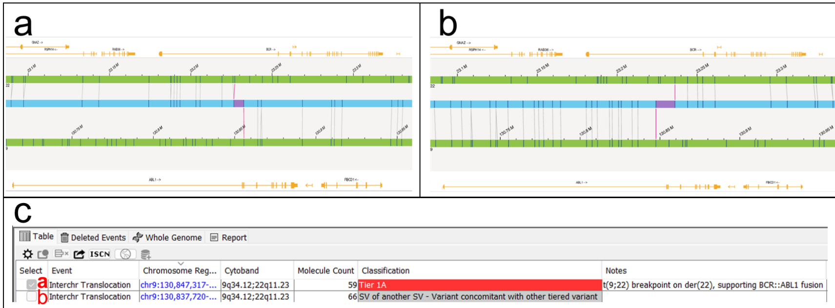
Figure 3. Case BNGOHM-0001054’s balanced t(9;22) and resulting SV calls, classifications. In top panels, Bionano Access shows center (blue) OGM consensus maps aligned partly to GRCh38 chromosome 22 (upper green track) and partly to chromosome 9 (lower green track). Reference gene annotations are shown in golden yellow. a. Map alignment showing the der(22) breakpoint, the configuration supporting a putative BCR::ABL1 gene fusion. b. Separate map alignment shows the reciprocal der(9) breakpoint. c. Display and classification of both breakpoints in VIA: Tier 1A for the der(22) from panel a., and SV of another SV – Variant concomitant with other tiered variant for the der(9) from panel b.
