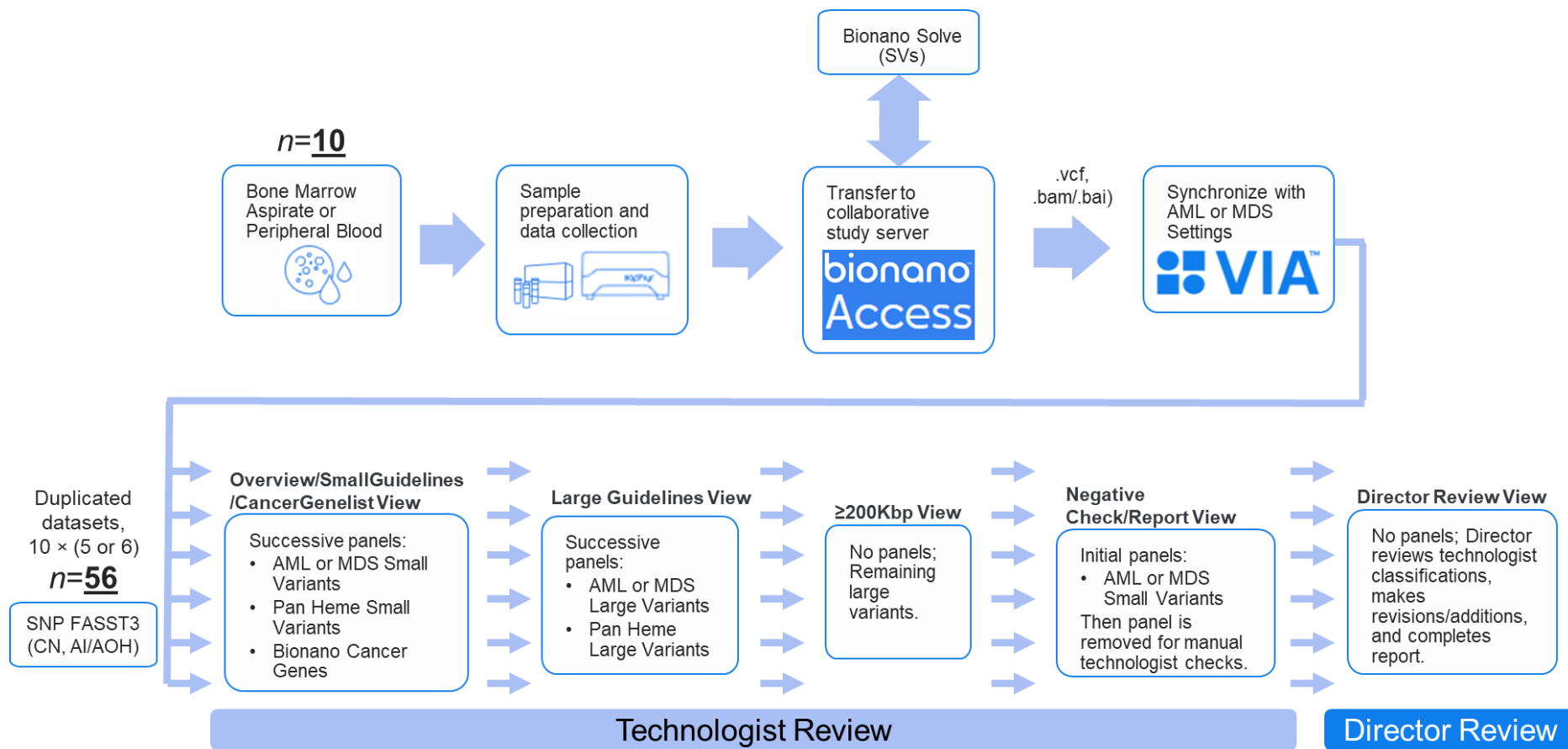
3 Figure 1. Data Flow and Replicate Analysis Framework. Ten bone marrow aspirate or blood samples from individuals with myeloid indications 4 were prepared for OGM data collection on the Saphyr System. Datasets targeting \geq 300\times effective coverage of GRCh38 were transferred to a 5 shared study server and analyzed using Solve 3.8 Rare Variant Analysis for .vcf (SVs), .bam/.bai outputs. These files were synced to a shared VIA 6 server and assigned an appropriate 300\times multiscale reference, duplicated into multiple copies for replicate review, and processed for CN and BAF 7 data using the SNP FASST3 algorithm. Each dataset then underwent five or six reviews, proceeding in two stages: Technologist review, which 8 consists of panel and filter application in the Overview/Small Guidelines/CancerGenelist, Large Guidelines, \geq 200\text{Kbp} , and Negative Check/Report 9 Views; and a subsequent Director review for final classification and summary report generation.
