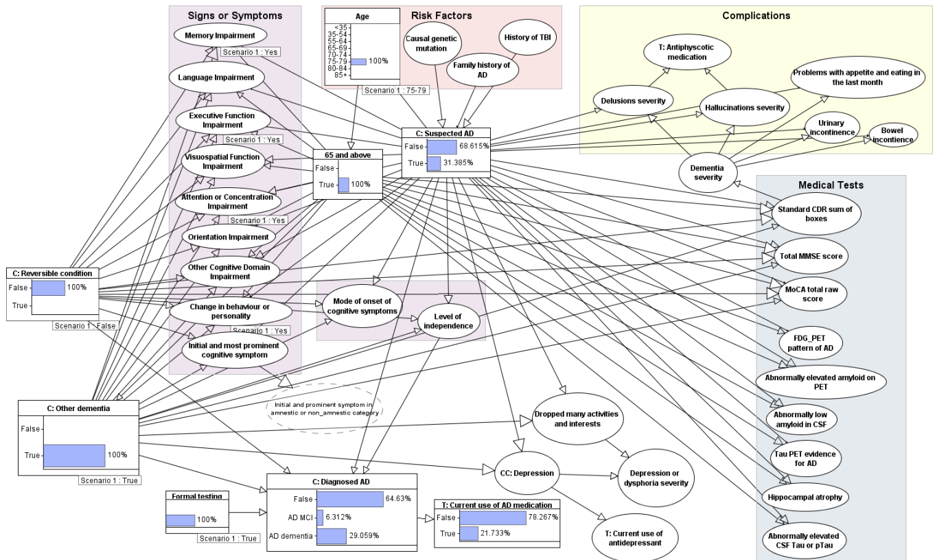
Figure 5. Bayesian network for clinical scenario A.
