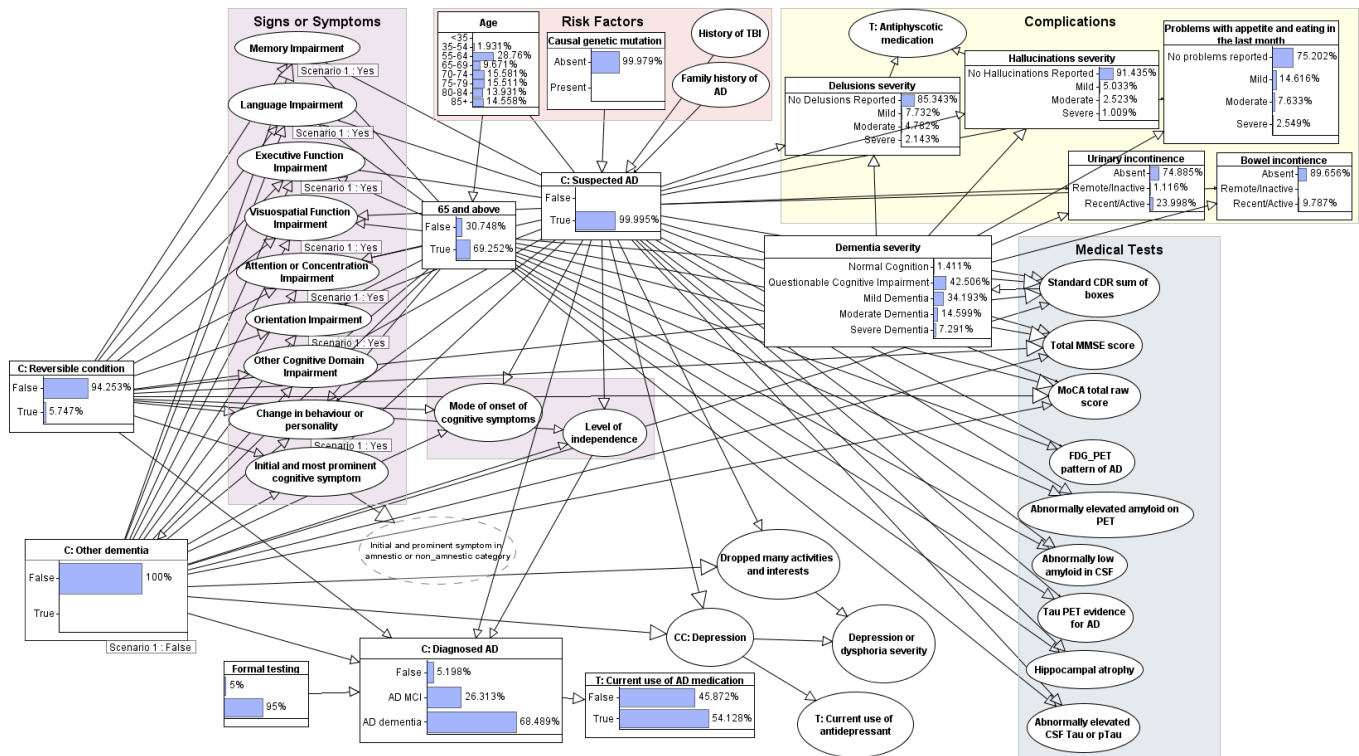
Figure 8. Bayesian network with all signs and symptoms observed. Other dementia is observed as False. Probabilities of complications are shown.
