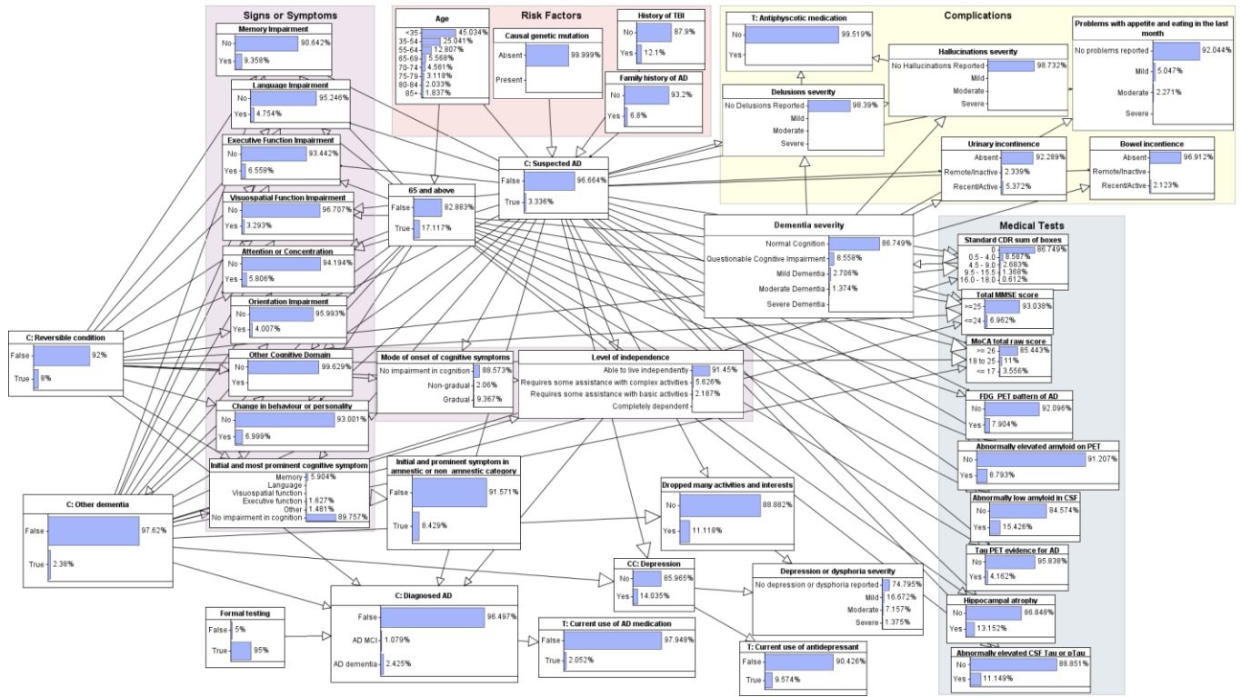
Figure 4. Full structure of the Bayesian network model for the diagnosis of Alzheimer's disease.
