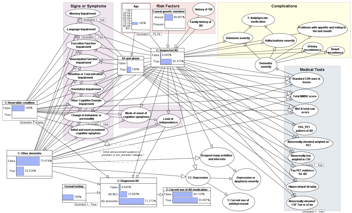
Figure 6. Bayesian network for clinical scenario B.
