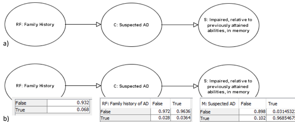
Figure 1. (a) A three-node Bayesian network. (b) A three-node Bayesian network with Node Probability Tables shown.
