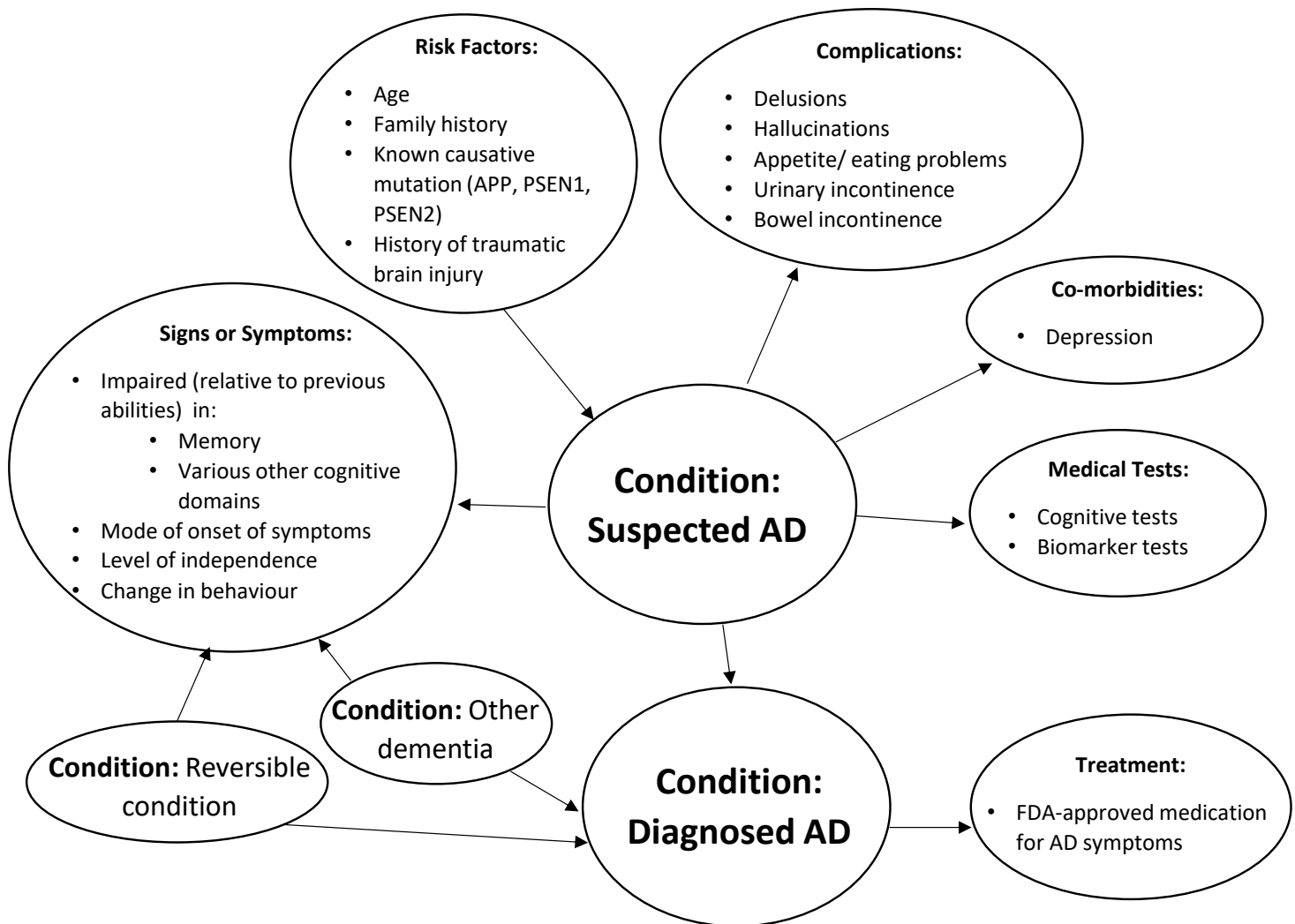
Figure 2. Simplified model schematic with the main variables included in the Bayesian network. Note that this is not the full model structure.
