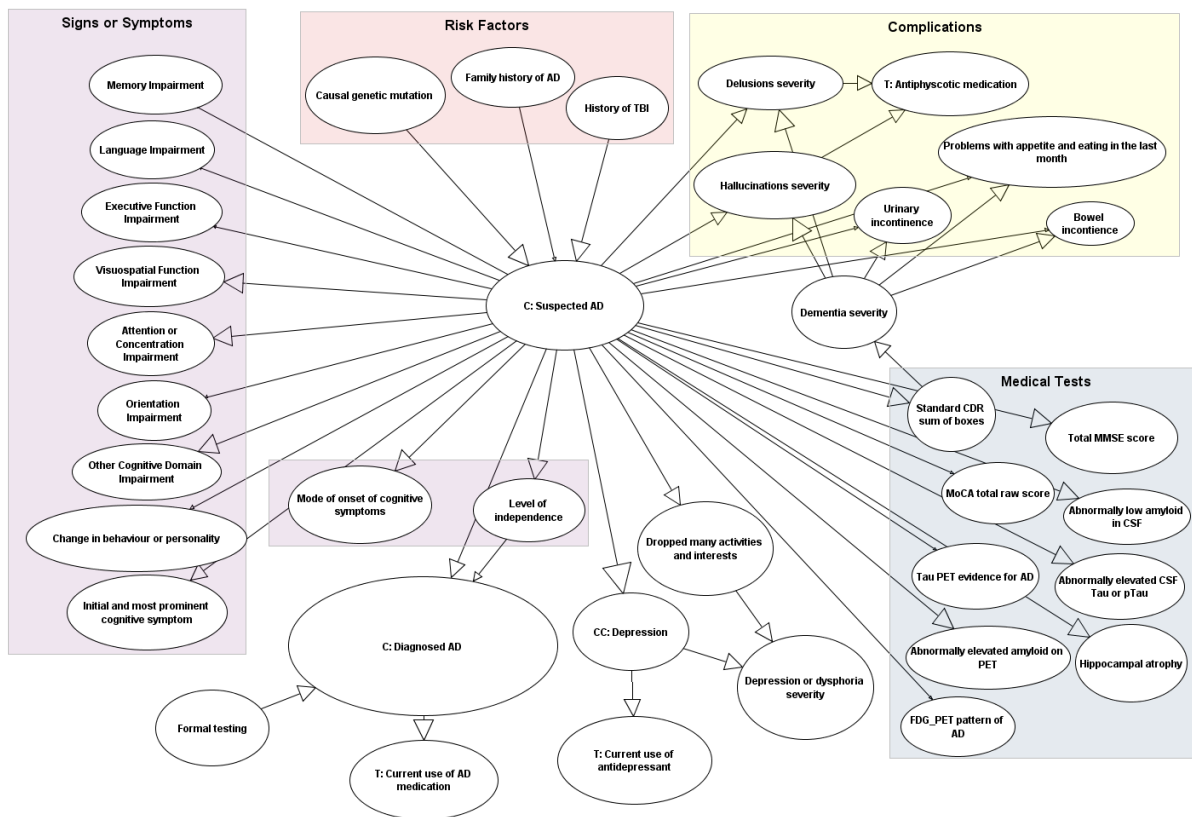
Figure 3. Full structure of the Bayesian network model for the diagnosis of Alzheimer's disease. The nodes 'Age', '65 and above', 'C: Other dementia' and 'C: Reversible condition' are hidden in the model to reduce the visual complexity.
