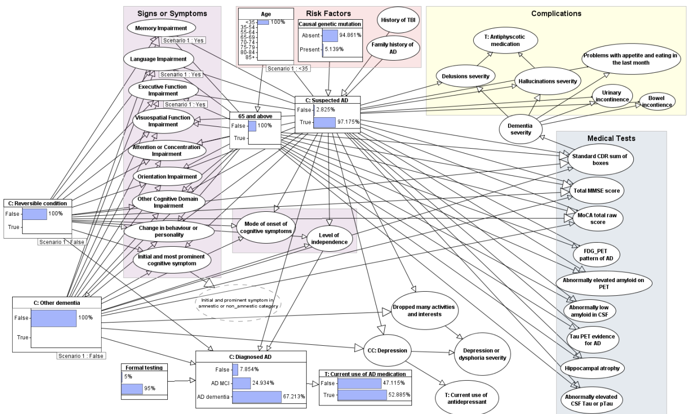
Figure 7. Bayesian network with age and certain signs or symptoms observed. Other conditions are ruled out (observed as False).
