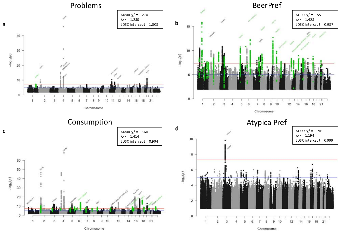
Figure 3. Manhattan plots of the latent factor genome-wide association (GWAS) results.
