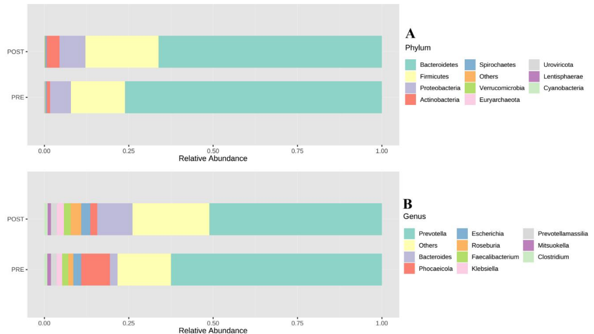
Figure.4: Differential Abundance across Phylum [A] and Genus [B] levels.
