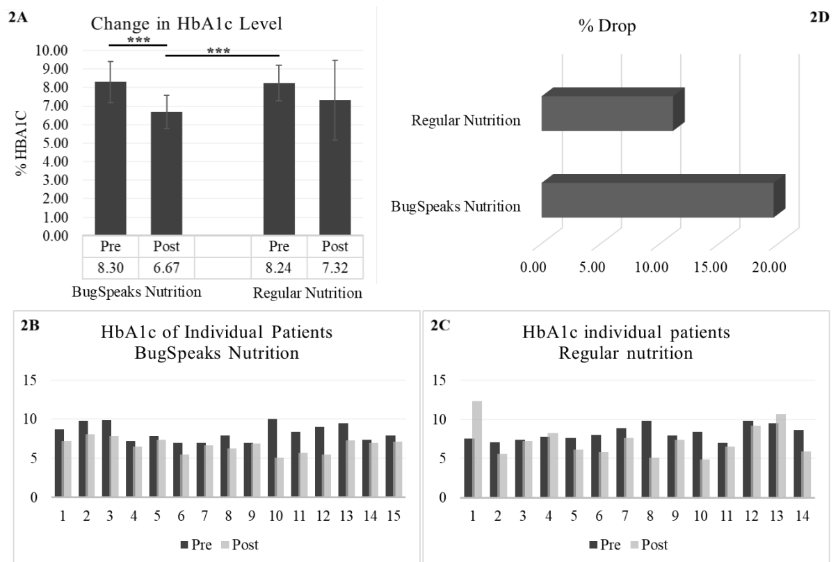
Figure 2: Change in HbA1c levels. A: Overall change in HbA1c levels across the arms, where ***p < 0.001 . B & C: Change in HbA1c levels in each individual, within the BugSpeaks personalized nutrition arm and the regular nutrition arm, respectively. D: Overall % drop between the two arms.
