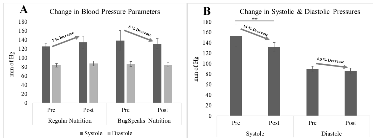
Figure 3: Change in Blood Pressure Parameters. A: Overall change in Systolic and Diastolic pressures across the comparing arms of Regular Nutrition and BugSpeaks Nutrition. B: Change in Systolic and Diastolic pressures within a sub-cohort of patients in BugSpeaks Nutrition Showing a significant reduction in Systole within the arm, with **p < 0.01 .
