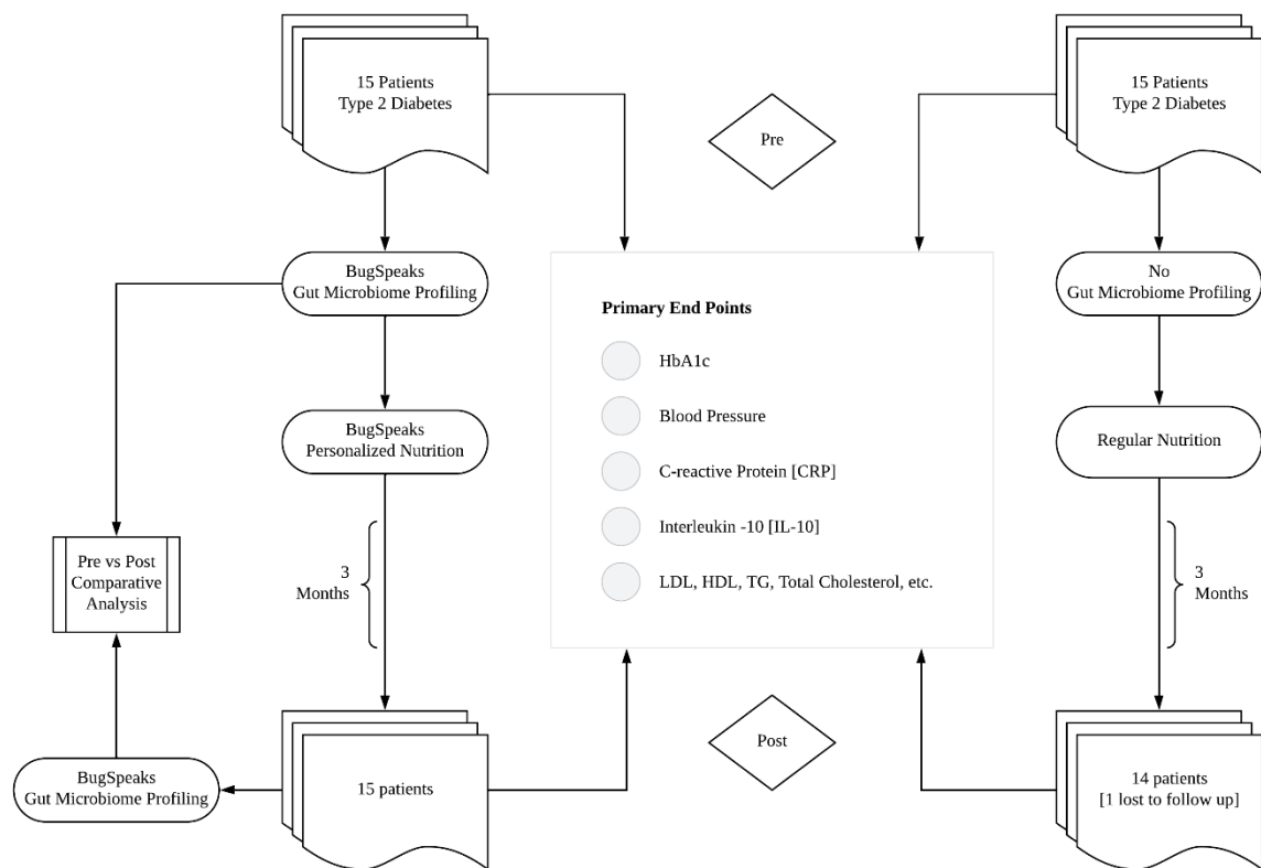
Figure 1: Study Design. A flow chart depicting the study design, with two arms of the study, list of clinical parameters evaluated as primary end points and the microbiome profiling for the intervention arm [left]
