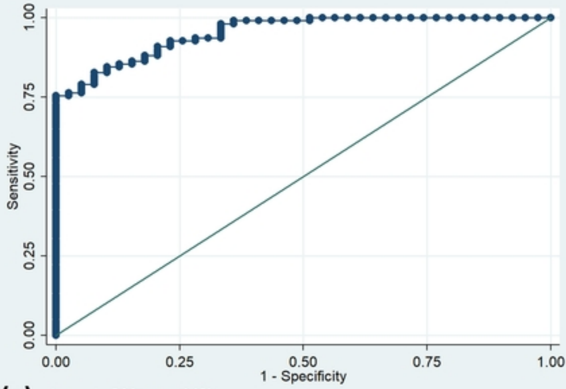
(a) Area under ROC curve = 0.9524
