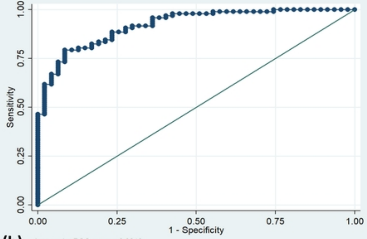
(b) Area under ROC curve = 0.9210
